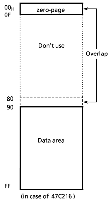
Figure 1-2. RAM addressing
