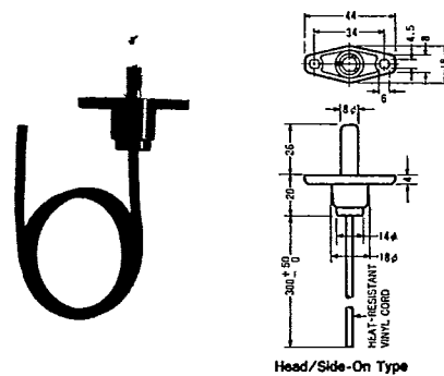
Head/Side-On Type
