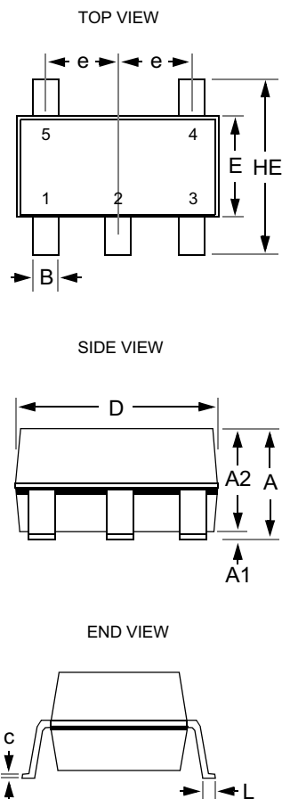
Package Dimensions for SC70-5
