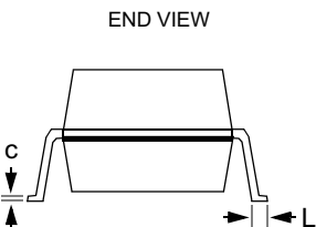
Package Dimensions for SC70-6.
