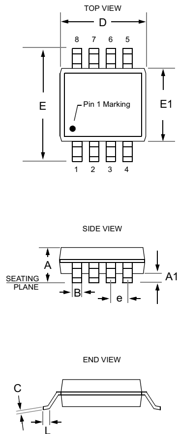
Package Dimensions for TSSOP-8
