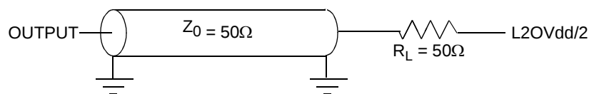
Figure 17. AC Test Load for the L2 Interface
