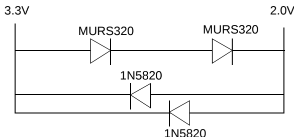
Figure 30. Example Voltage Sequencing Circuit
