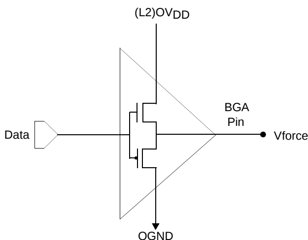
Figure 32. Alternate Driver Impedance Measurement Circuit
