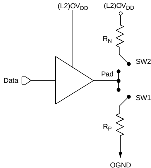
Figure 31. Driver Impedance Measurement Circuit
