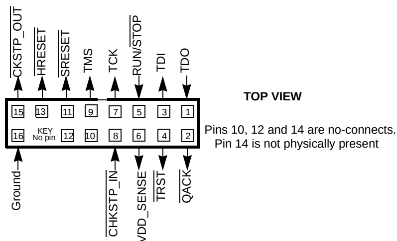
Figure 24. COP Connector Diagram
