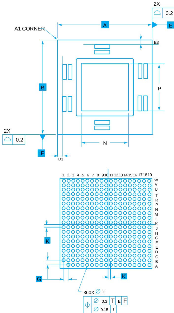
Figure 28. Mechanical Dimensions and Bottom Surface Nomenclature of PC755B (CI-CGA)
