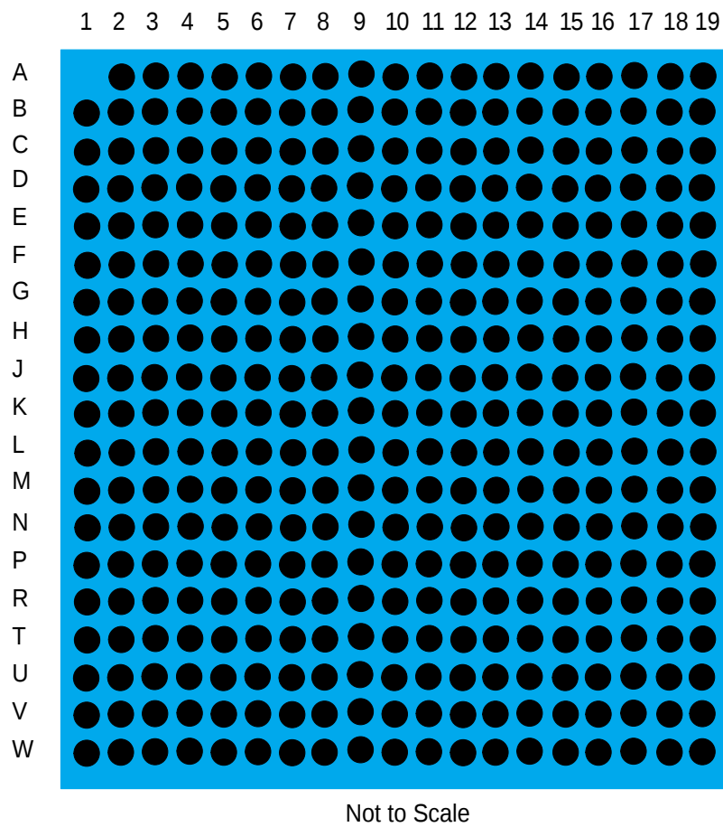
Figure 3. Pinout of the PC755B, 360 PBGA, CBGA and CI-CGA Packages as Viewed from the Top Surface
