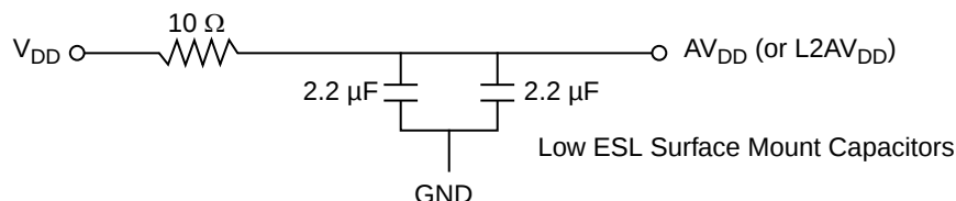
Figure 29. PLL Power Supply Filter Circuit
