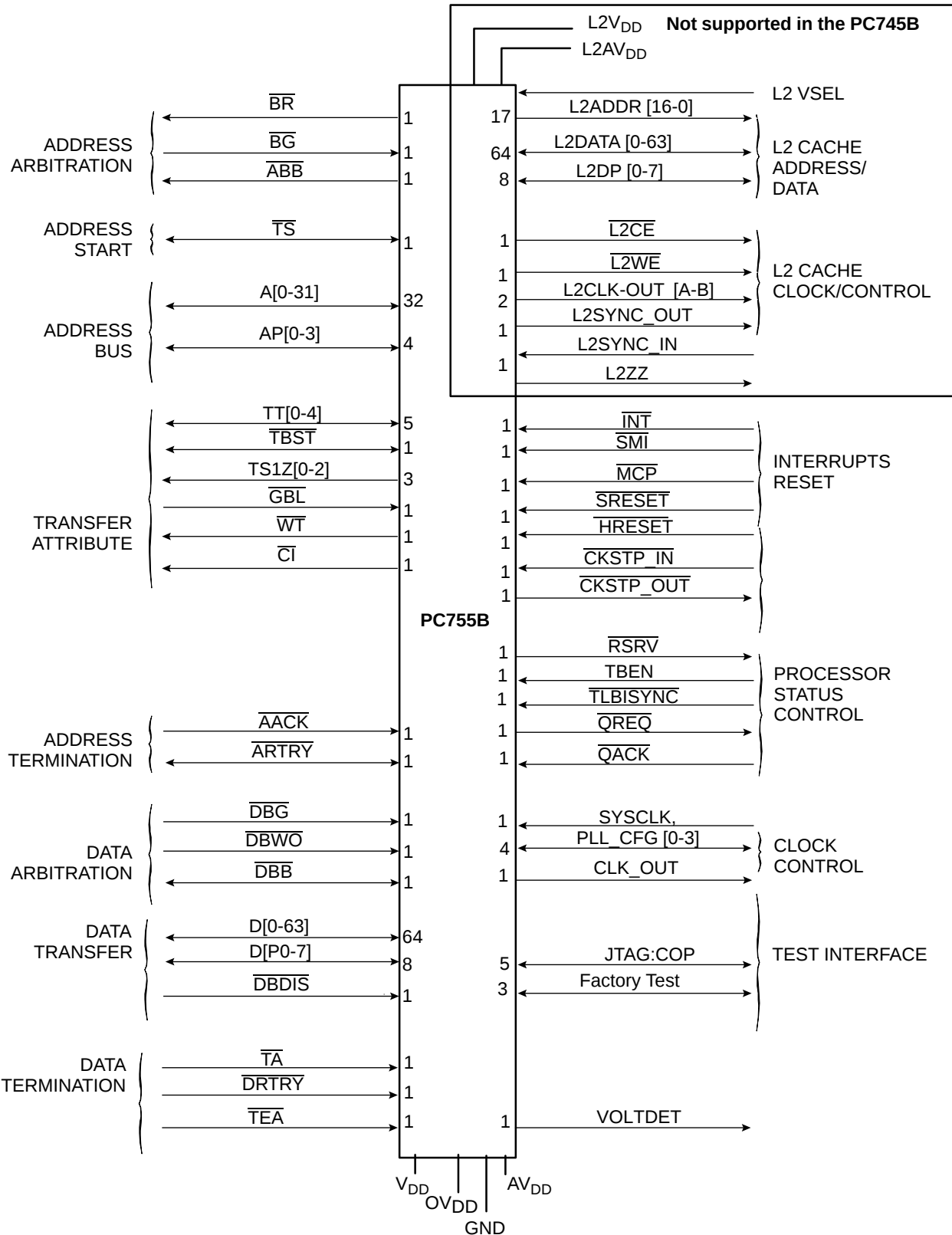
Figure 4. PC755B Microprocessor Signal Groups
