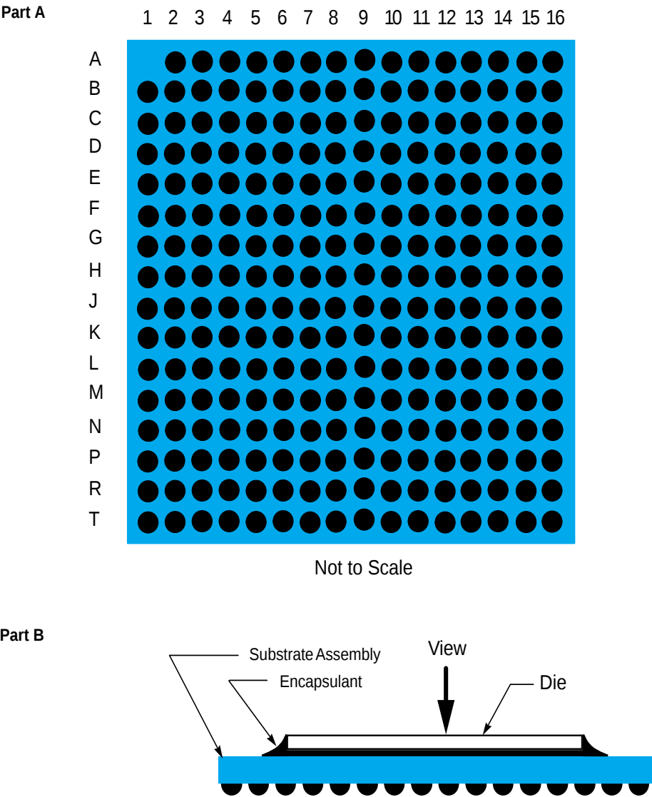
Figure 2. Pinout of the PC745B, 255 PBGA Package as Viewed from the Top Surface
