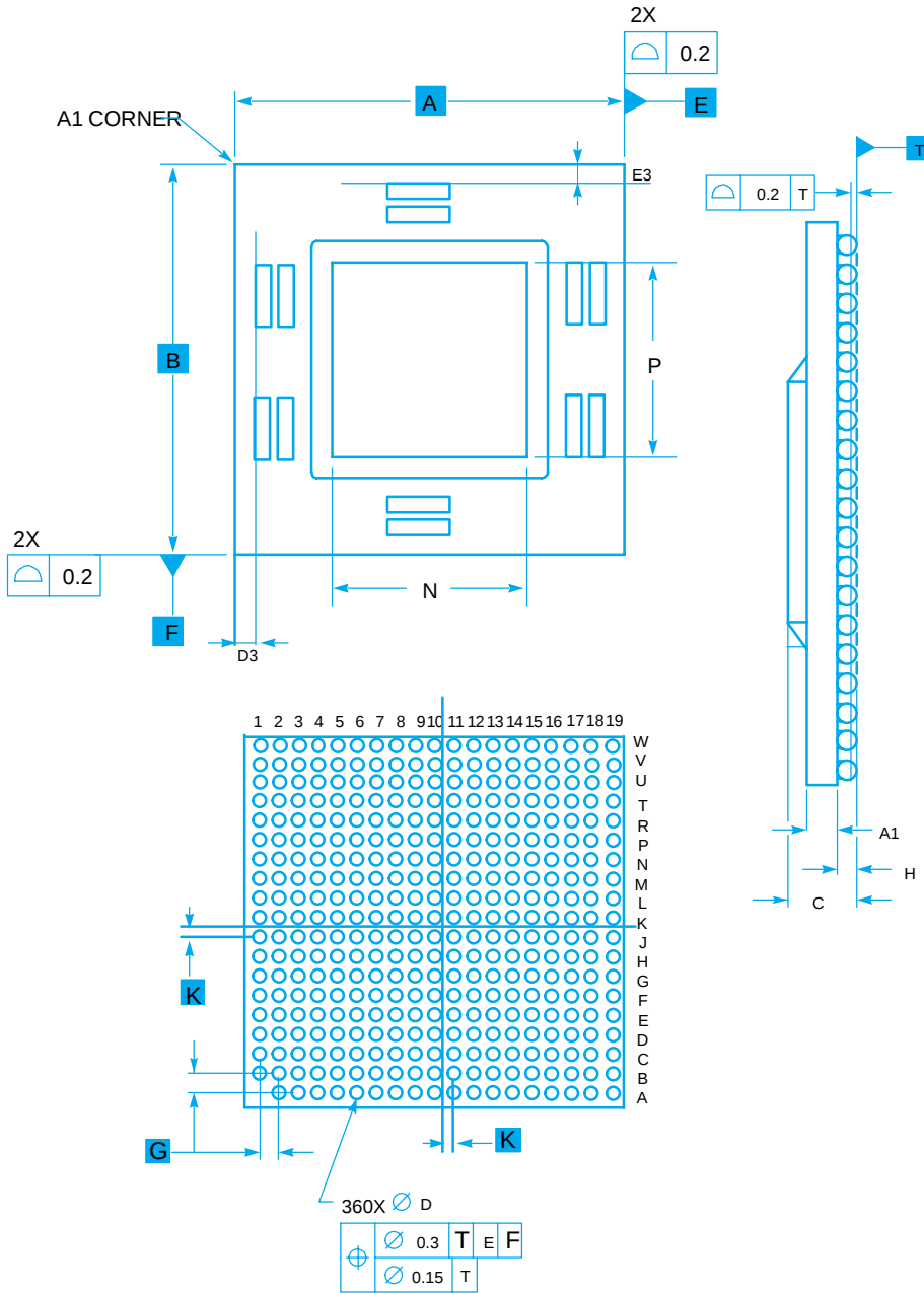
Figure 27. Mechanical Dimensions and Bottom Surface Nomenclature of PC755B (CBGA)
