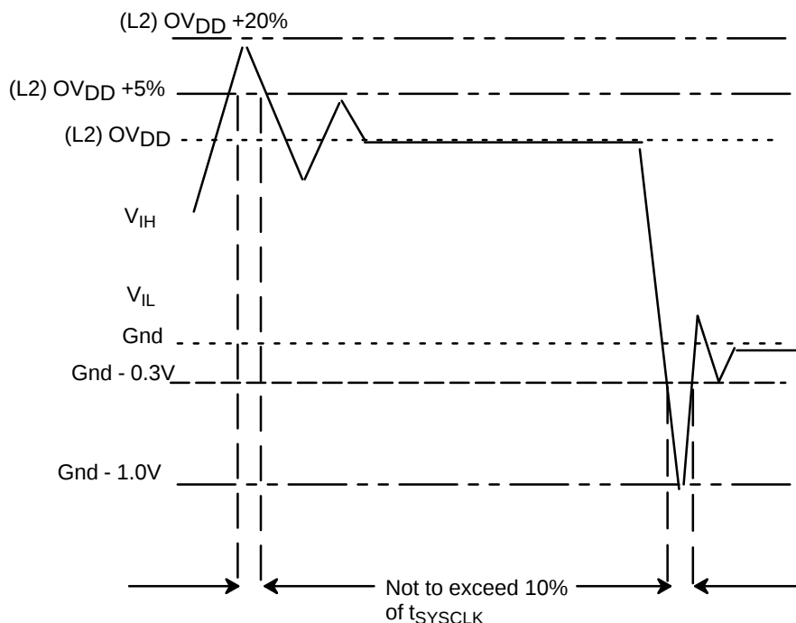
Figure 5. Overshoot/Undershoot Voltage
