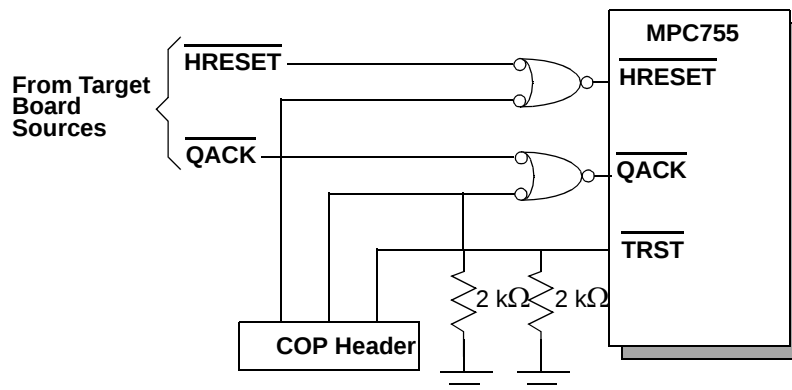
Figure 23. Suggested \overline{\text{TRST}} Connection
