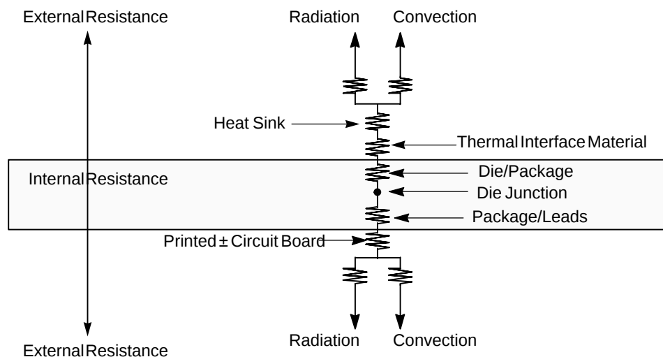
Figure 6. C4 Package with Heat Sink Mounted to a Printed-circuit Board
