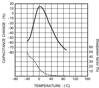
Fig.5 Capacitance-temperature characteristics
