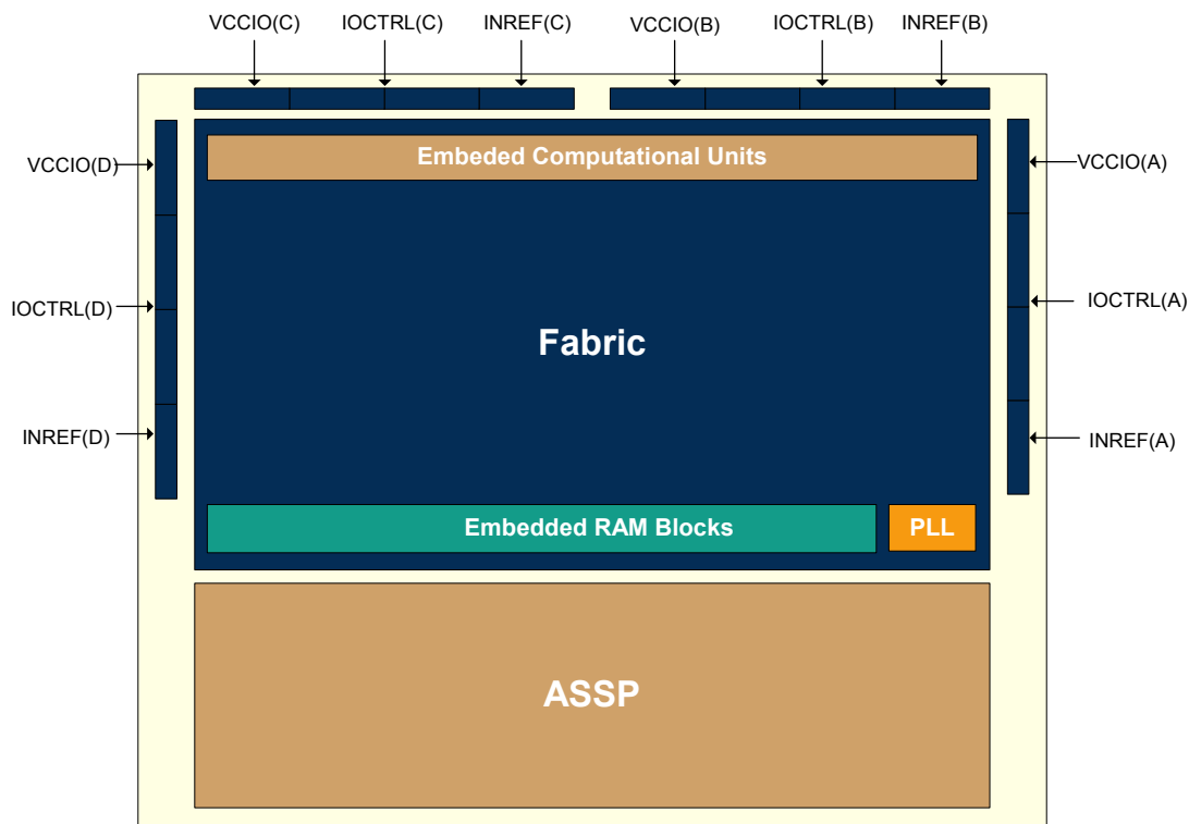
Figure 19: Multiple I/O Banks
