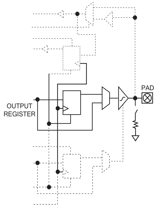
Figure 53: QL903M Output Register Cell
