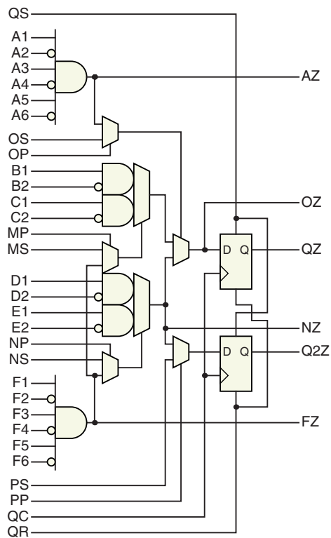
Figure 40: QL903M Logic Cell
