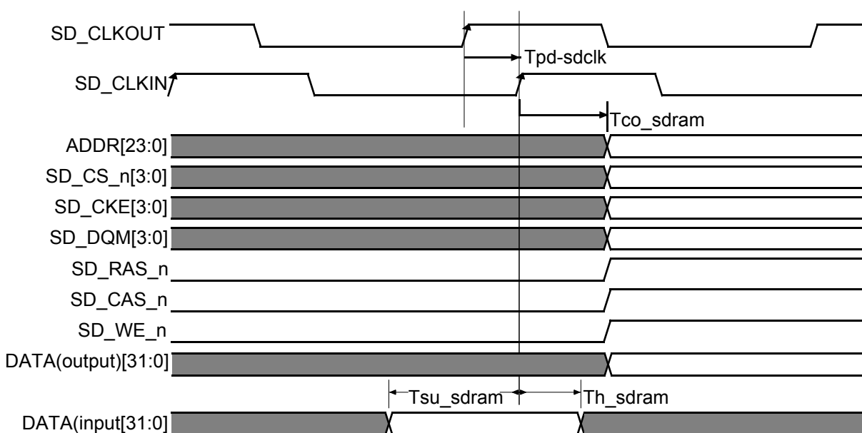
Figure 33: SDRAM Waveforms
