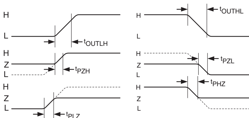
Figure 54: QL903M Output Register Cell Timing
