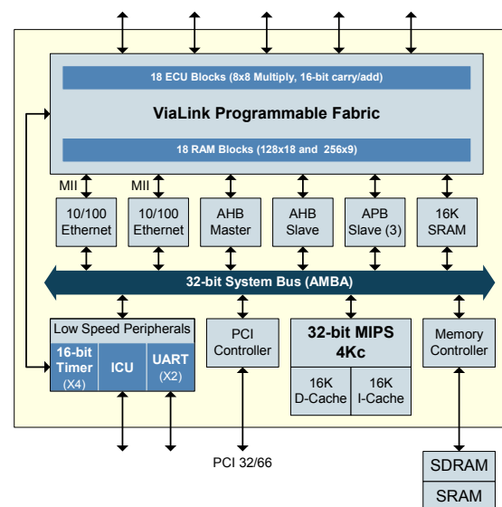
Figure 1: QL903M Block Diagram
