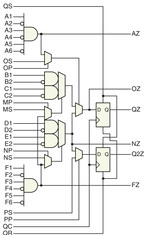
Figure 10: QL903M Logic Cell
