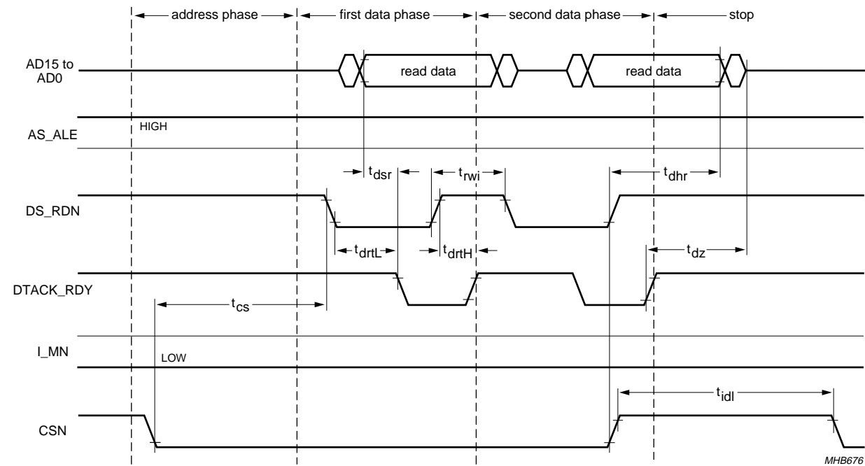
Fig.17 Motorola-style protocol mode (external address decoding).
