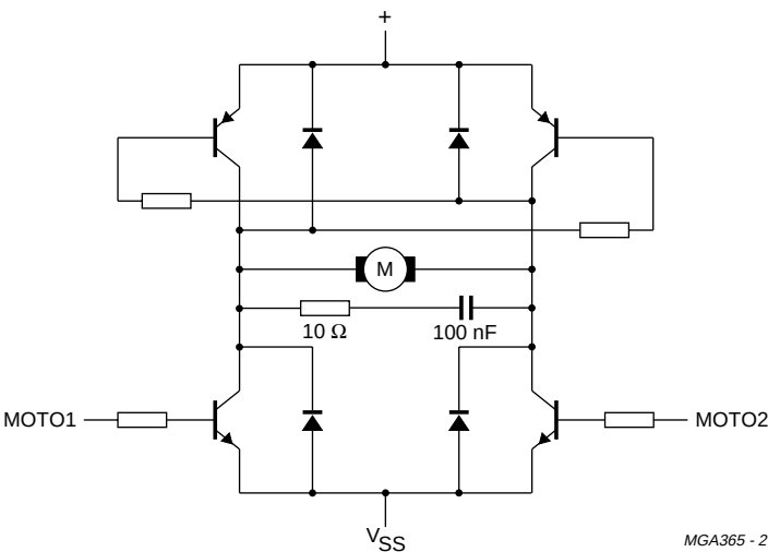
Fig.16 Motor 2-line PWM mode application diagram.
