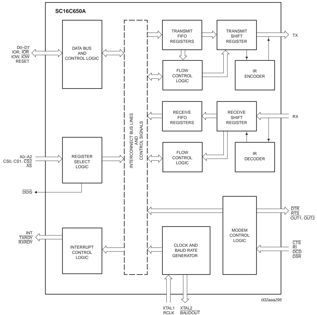
Fig 1. Block diagram.
