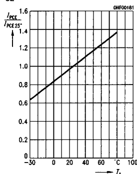
Photocurrent I_{\text{PCE}}/I_{\text{PCE}25^\circ} = f(T_A) , V_{\text{CE}} = 5 \text{ V}
