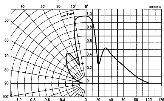
Directional characteristics S_{\text{rel}} = f(\varphi)
