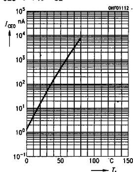
Dark current
