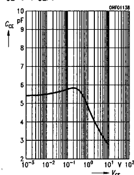
Collector-emitter capacitance
