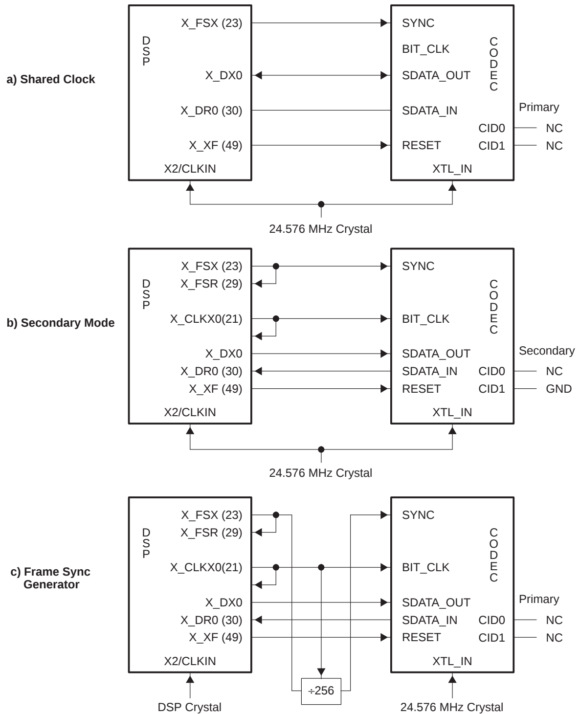
Figure 1–5. DSP-CODEC Configurations
