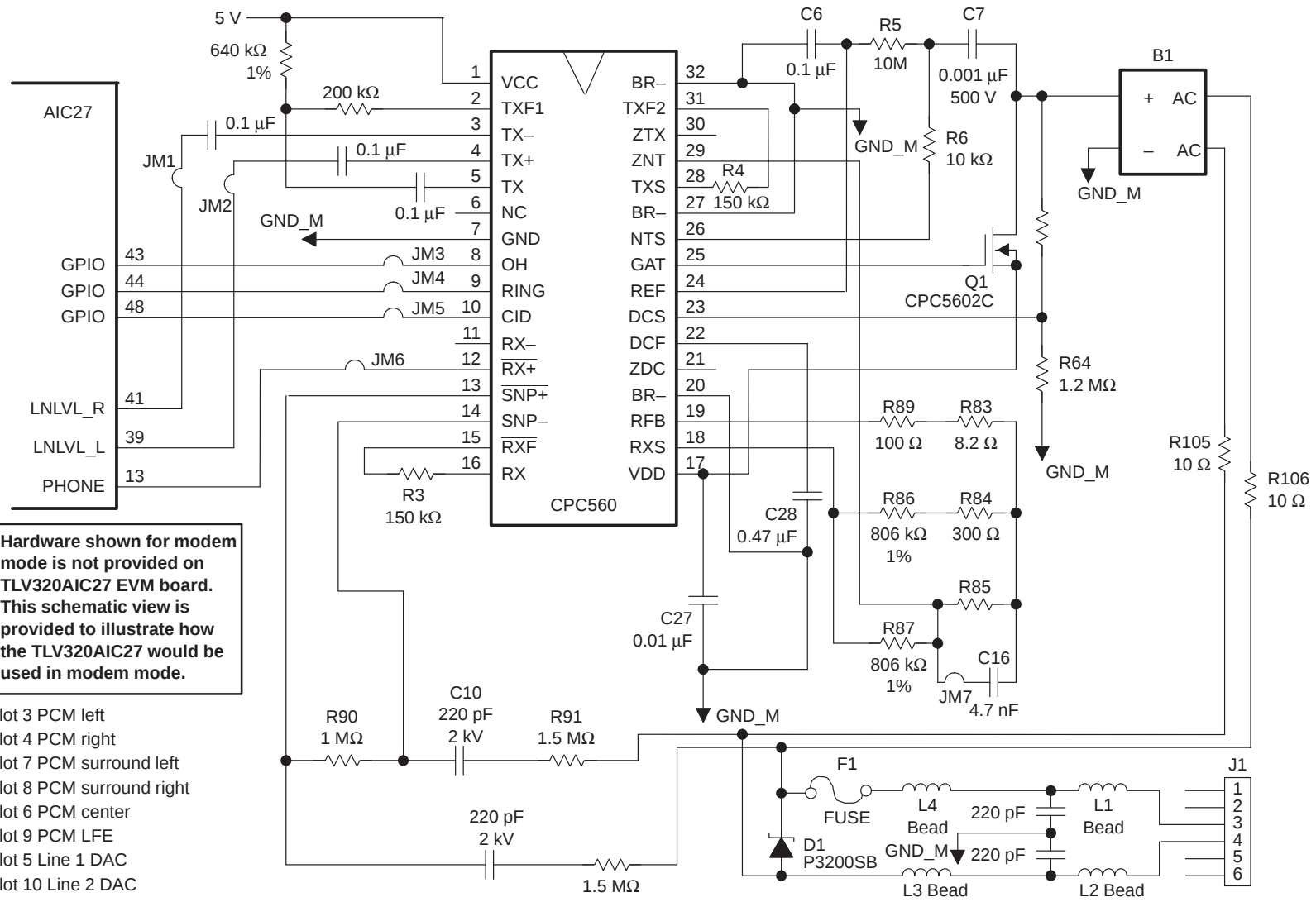
Figure 2–4. Modem Mode
