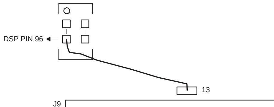
Figure 1–3. Pin 96 to DSK J9–13 Connection
