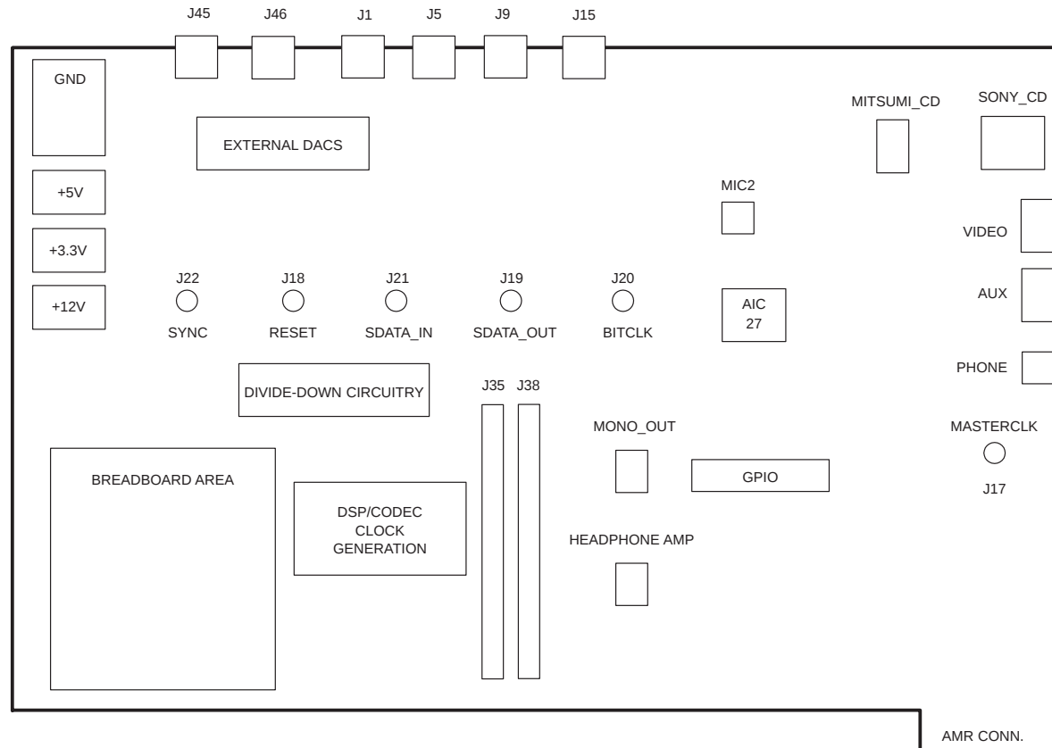
Figure 1–2. EVM Layout
