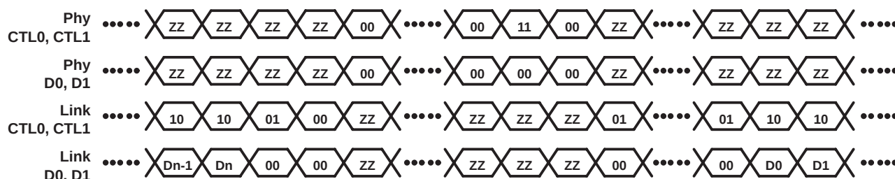
Figure 7. Transmit Timing Waveforms
