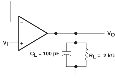
Figure 1. Unity-Gain Amplifier
