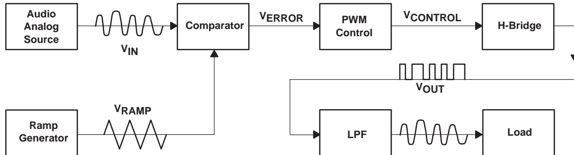
Figure 3–5. Class-D Functional Diagram
