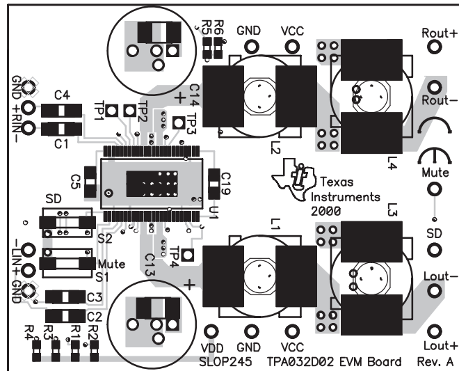
Figure 3–20. TPA032D02 Class-D EVM Top Assembly
