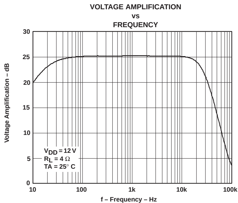
Figure 3–11. Class-D Amplifier Frequency Response at 4 \Omega
