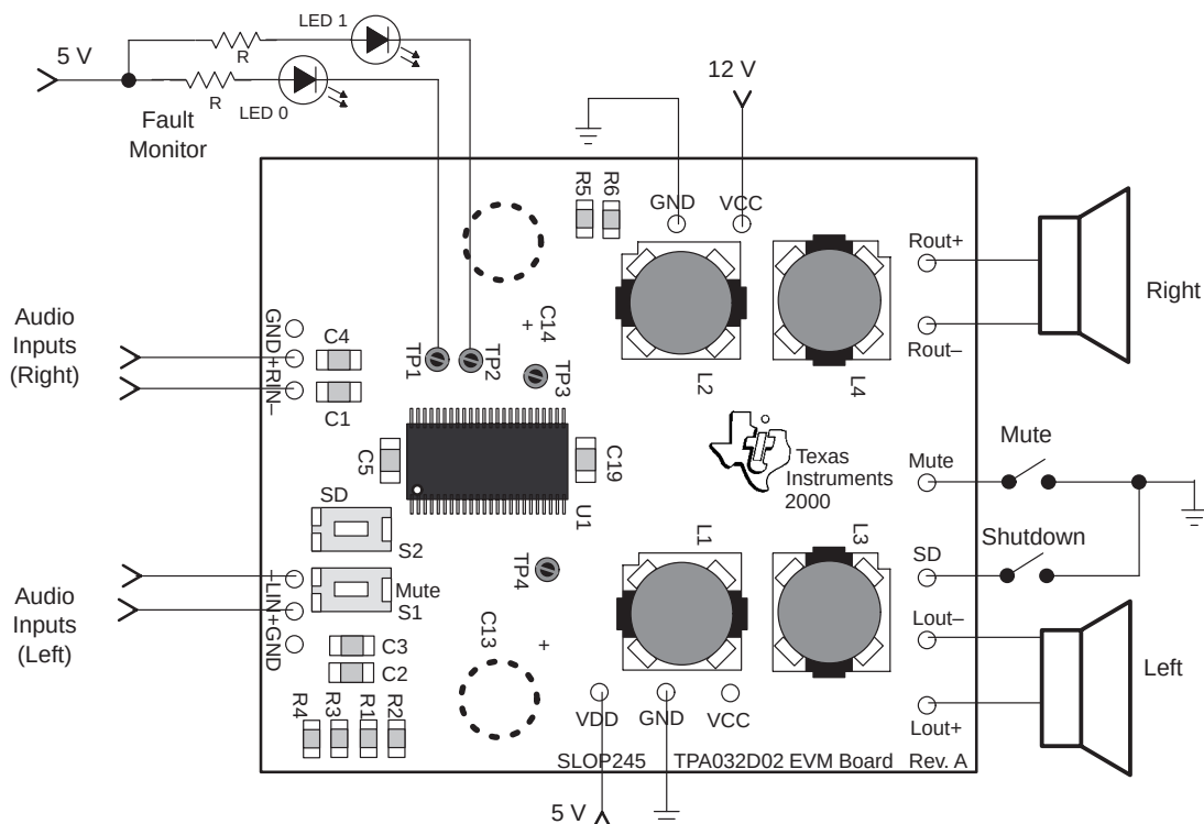
Figure 3–10. TPA032D02 Class-D EVM Stand-Alone Connections for Stereo BTL Output
