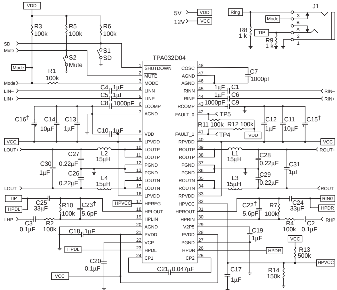
Figure 3–23. TPA032D04 Class-D EVM Schematic Diagram
