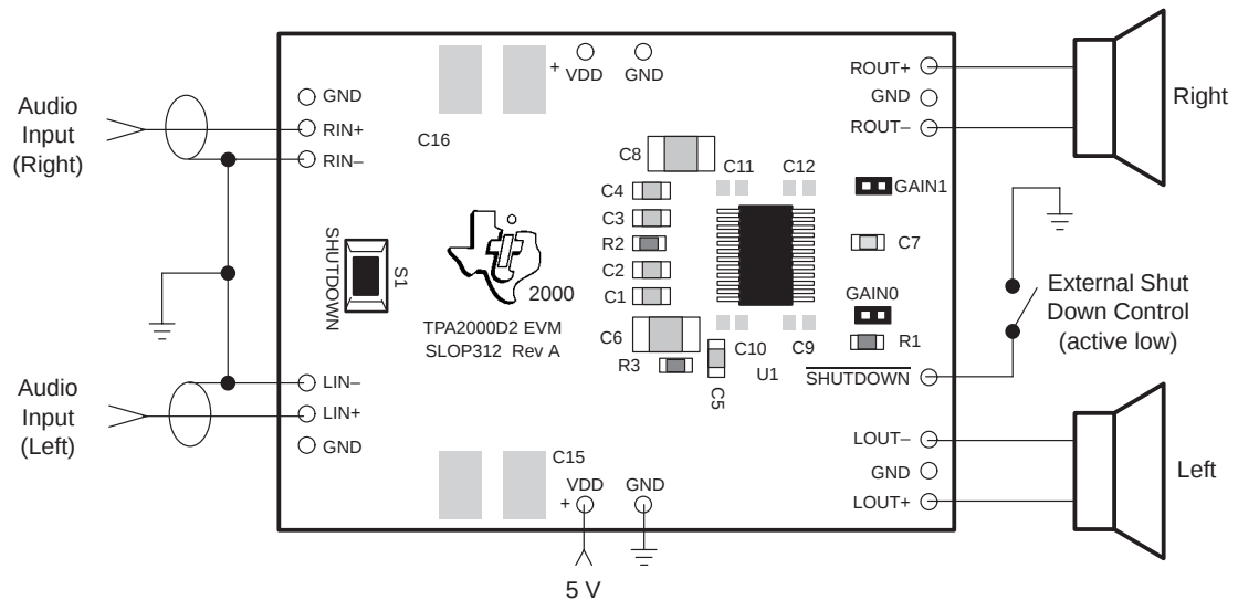
Figure 3–10. TPA2000D2 EVM Connected for Stereo Output
