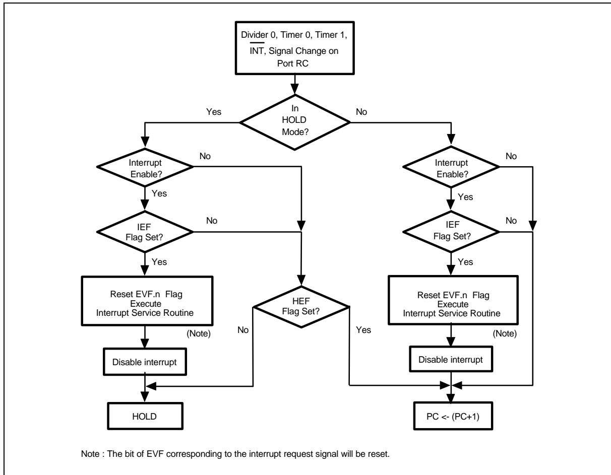
Figure 8. Hold Mode and Interrupt Operation Flow Chart
