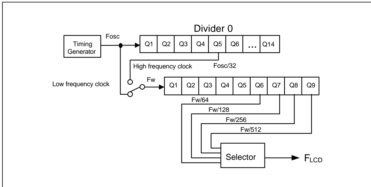
Figure 11. LCD Alternating Frequency ( F_{LCD} ) Circuit Diagram
