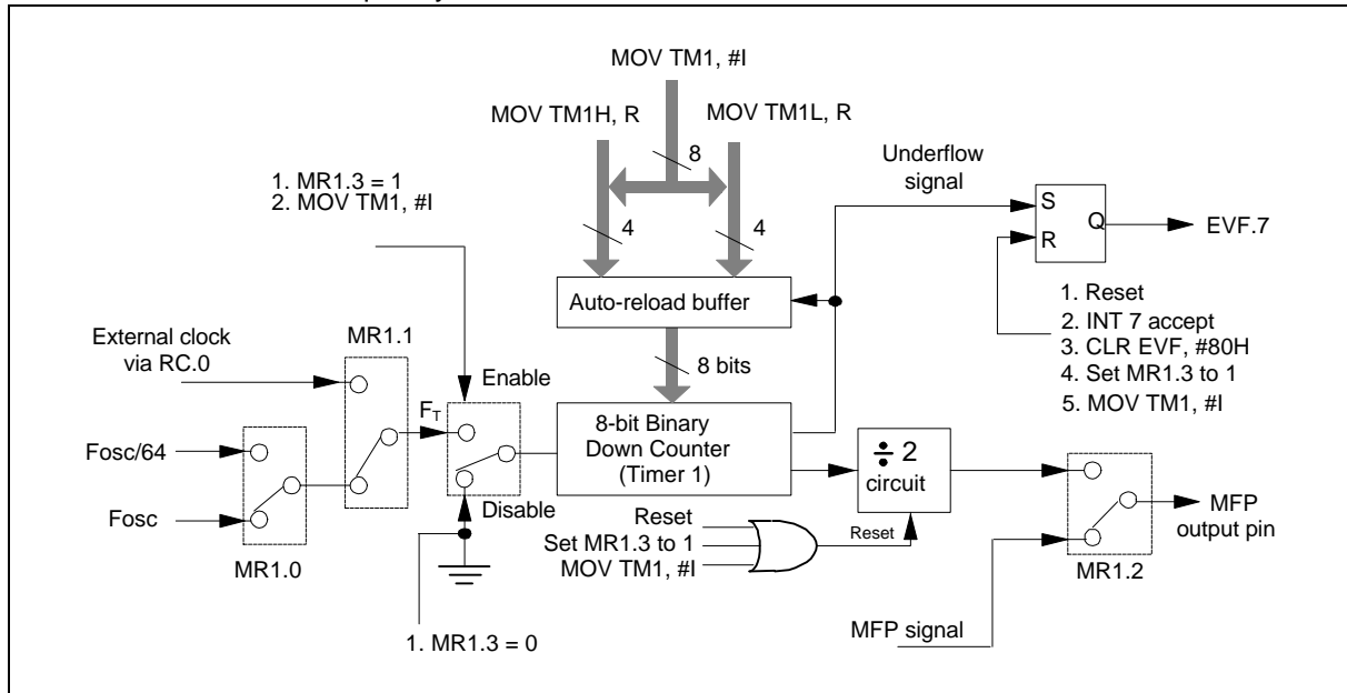
Figure 6. Organization of Timer 1
