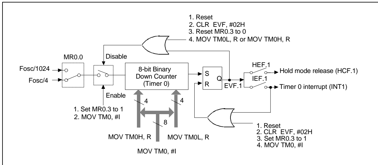
Figure 5. Organization of Timer 0
