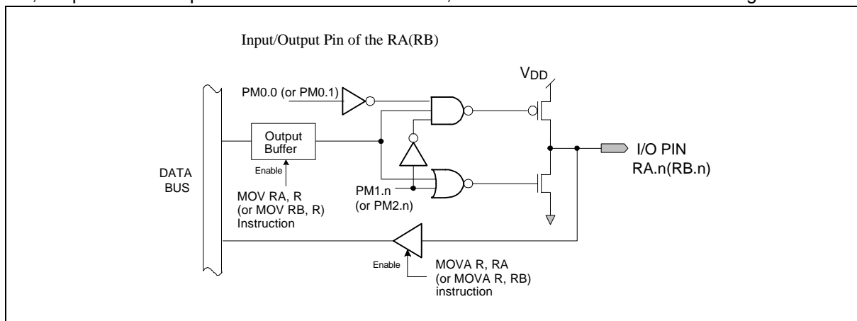
Figure 9. Architecture of Input/Output Pins
