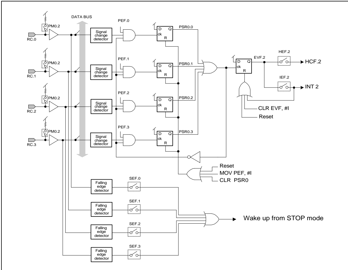
Figure 10. Architecture of Input Ports RC
