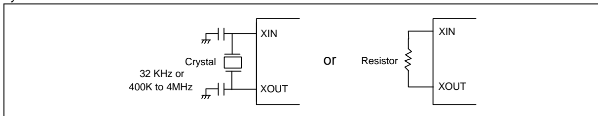
Figure 3. Oscillator Configuration
