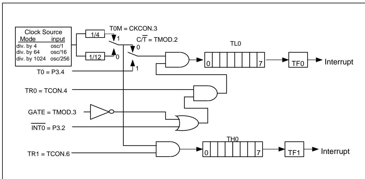
Figure 13. Timer/Counter 0 Mode 3
