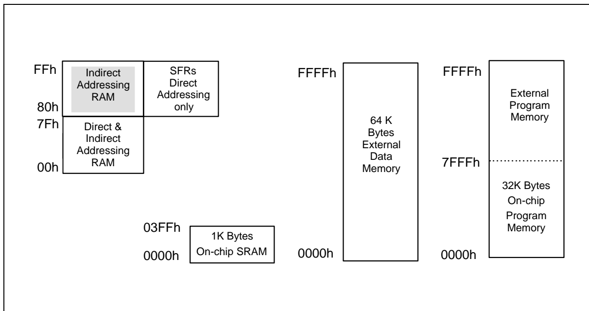
Figure 1. Memory Map
