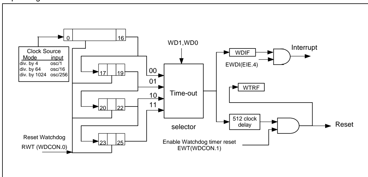
Figure 19. Watchdog Timer
