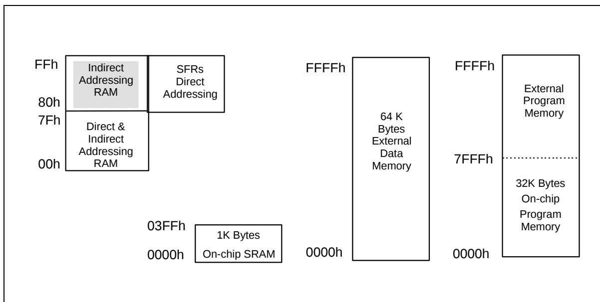
Figure 1. Memory Map
