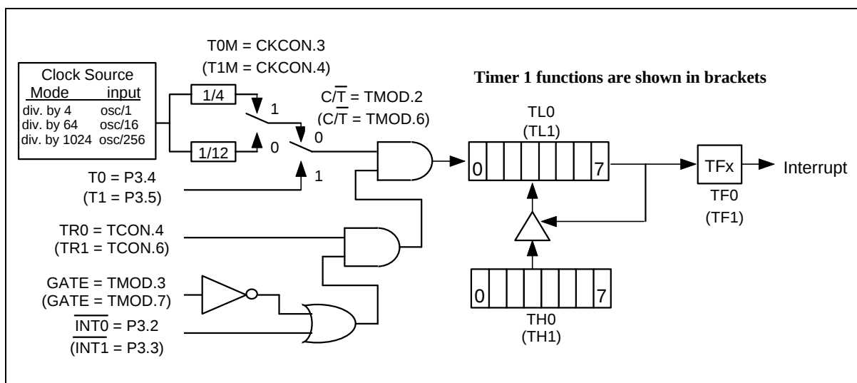
Figure 12. Timer/Counter Mode 2.
