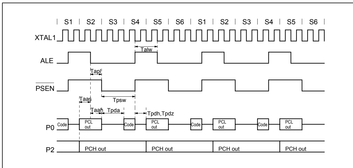
Figure 6. External Program Memory Fetch Cycle
