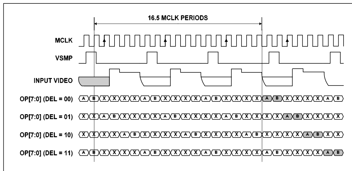
Figure 19 Mode 2 Operation
