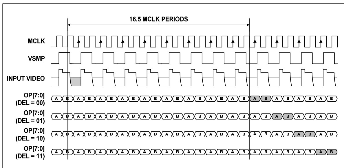
Figure 21 Mode 4 Operation
