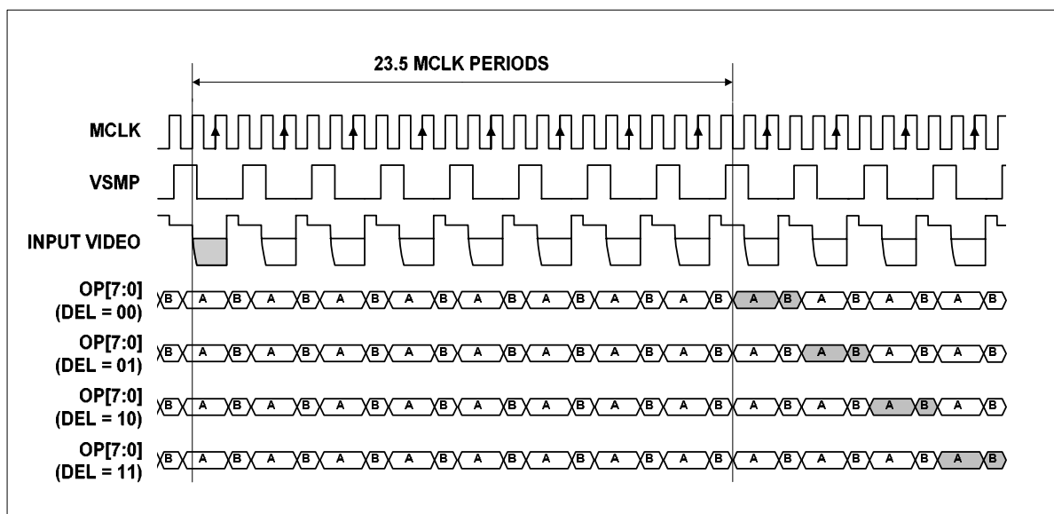
Figure 20 Mode 3 Operation
