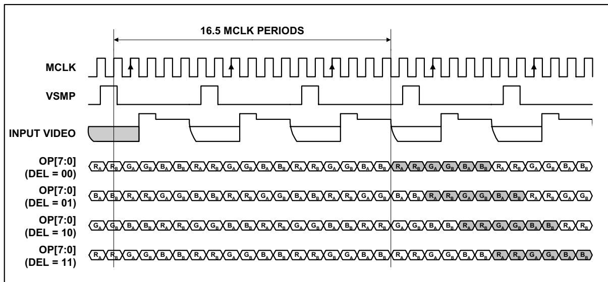
Figure 18 Mode 1 Operation
