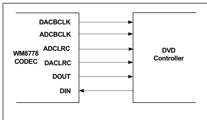
Figure 9 Master Mode
