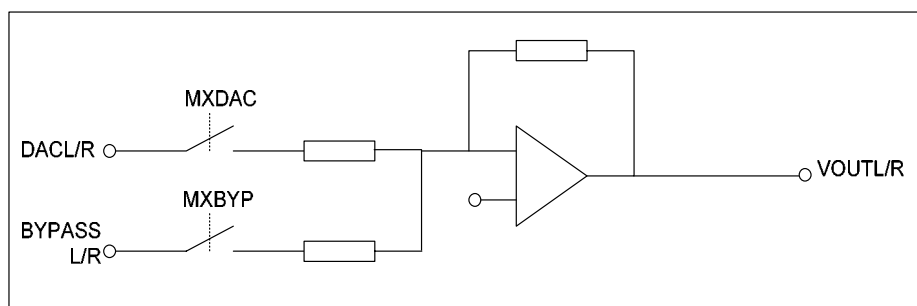
Figure 22 MX[2:0] Output Select
