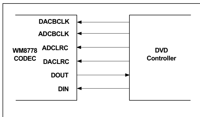
Figure 8 Slave Mode
