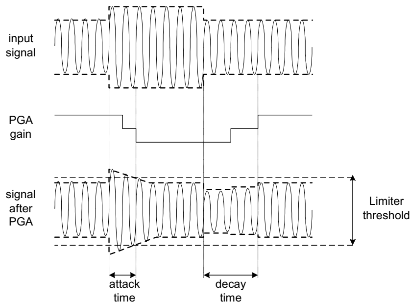
Figure 20 Limiter Operation
