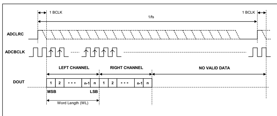
Figure 14 DSP Early Mode Timing Diagram – ADC Data Output
