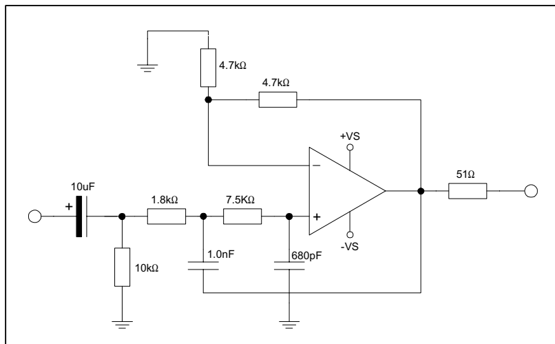
Figure 36 Recommended Post DAC Filter Circuit
