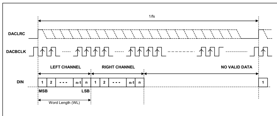
Figure 15 DSP Late Mode Timing Diagram – DAC Data Input
