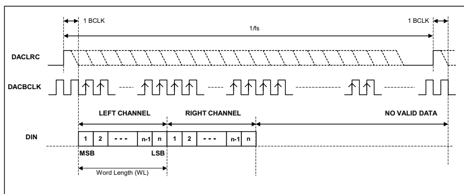
Figure 13 DSP Early Mode Timing Diagram – DAC Data Input
