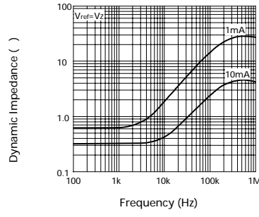
Dynamic Impedance v Frequency
