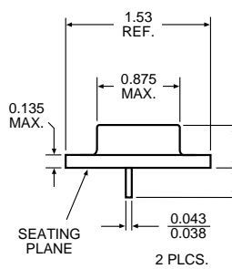
OM1325NKM Pin 1 - Adjust Pin 2 - Output Case - Input
