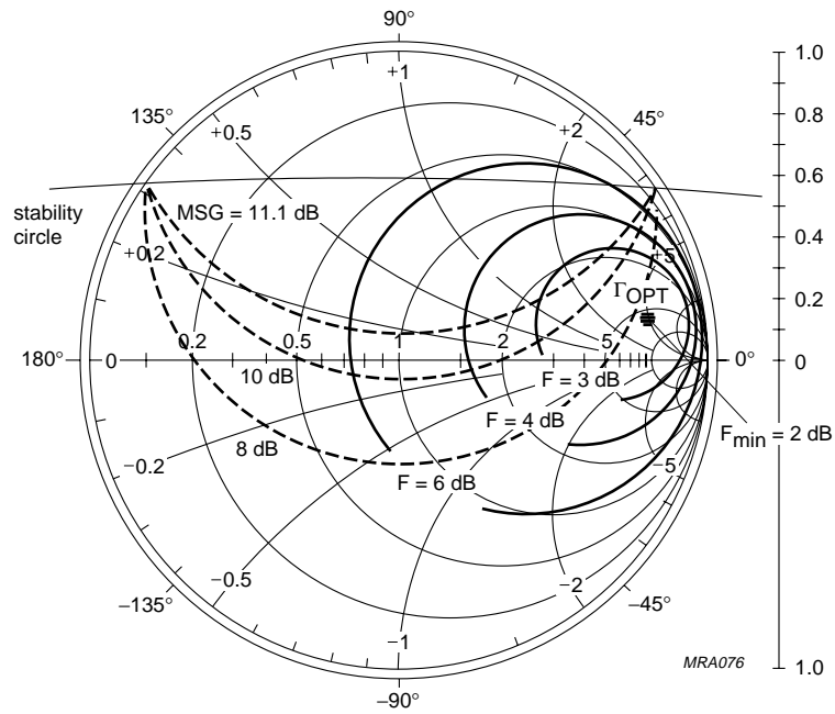
Fig.13 Noise circle.
