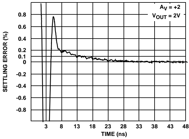
FIGURE 23. SETTLING RESPONSE
