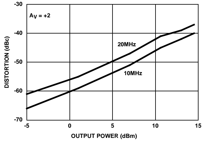
FIGURE 24. SECOND HARMONIC DISTORTION vs P_{OUT}
