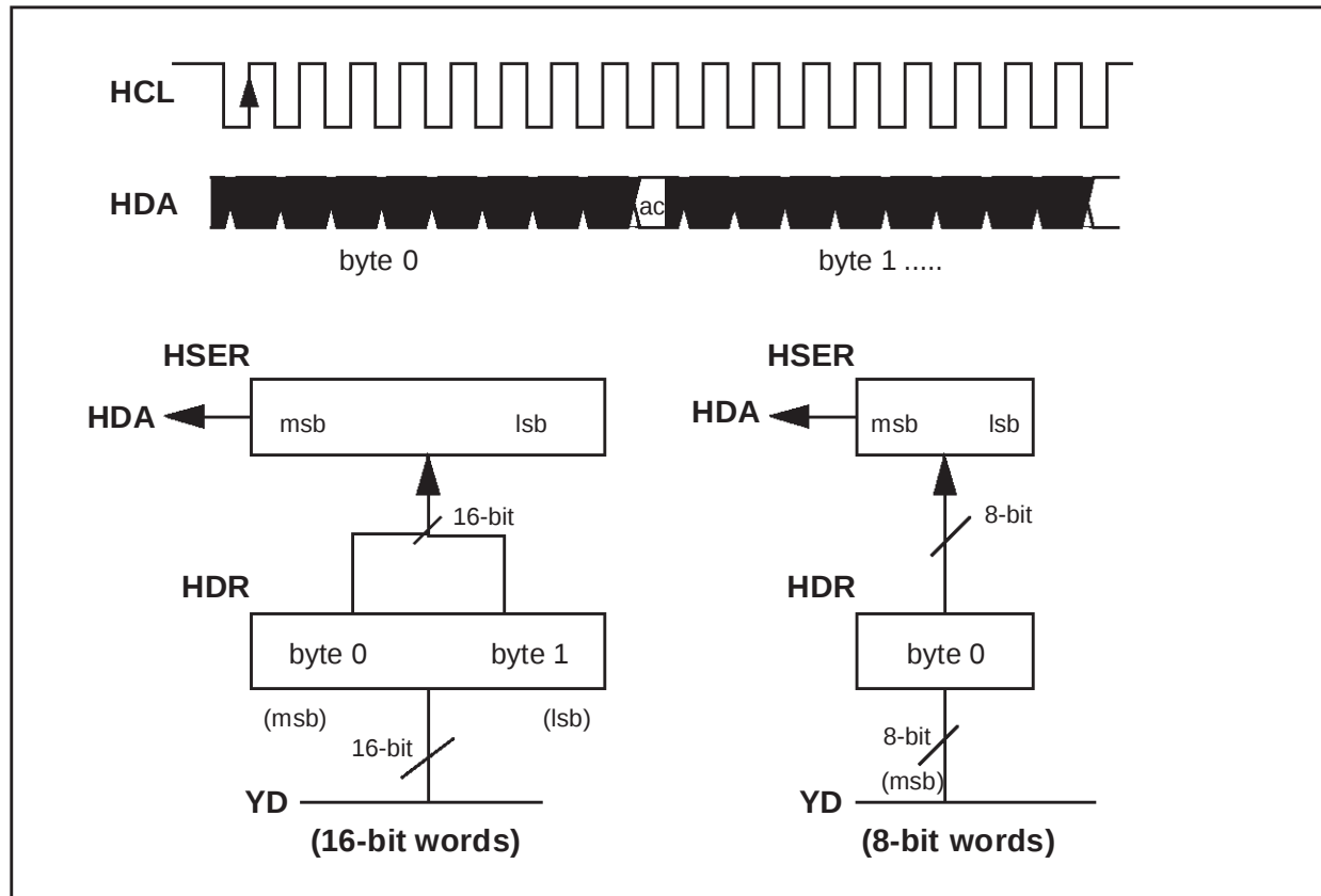
Figure 4.2 Host interface data exchange, send mode
