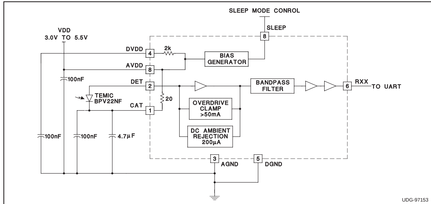
Figure 1. Typical Application of the UCC5341
