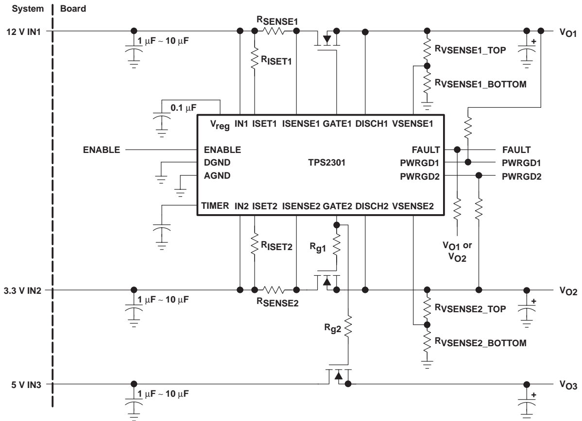
Figure 28. Three-Channel Application
