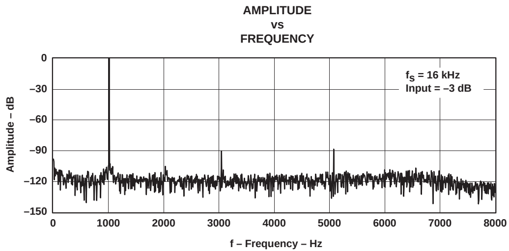
Figure 5-4. FFT-ADC Channel, f_s = 16 \text{ kHz} , Input = -3 dB
