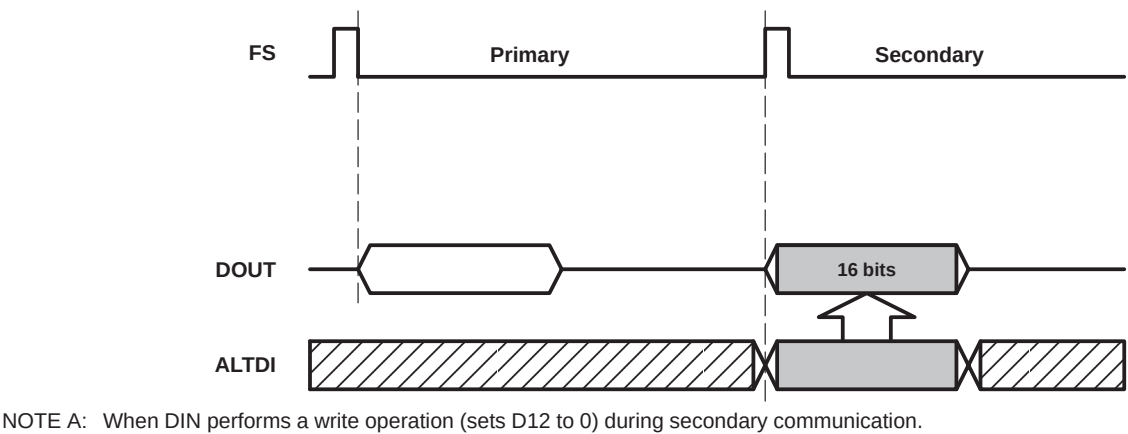
Figure 2–6. Event Monitor Mode Timing
