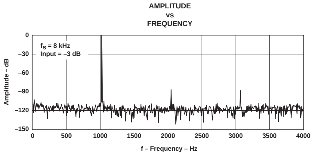
Figure 5-5. FFT-DAC Channel, f_s = 8 \text{ kHz} , Input = -3 dB
