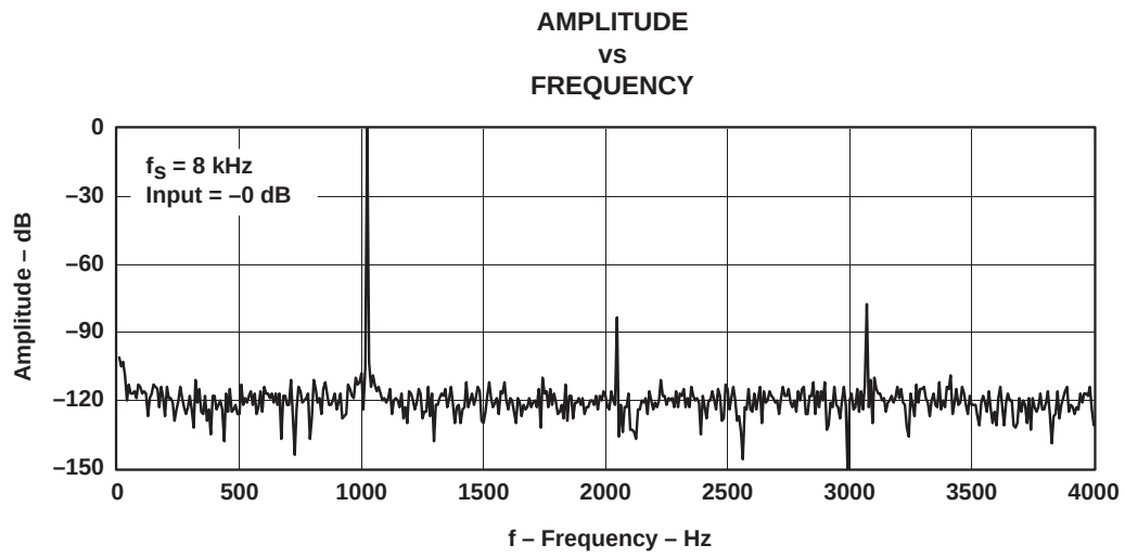
Figure 5-9. FFT-DAC Channel, f_s = 8 \text{ kHz} , Input = 0 dB
