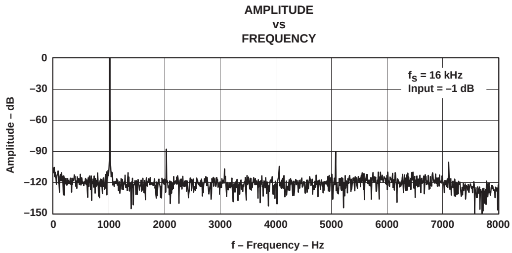
Figure 5-8. FFT-ADC Channel, f_s = 16 \text{ kHz} , Input = -1 dB
