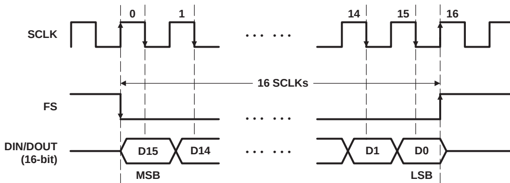
Figure 2–11. Timing Diagram for the FS Frame Mode (M1M0 = 11)
