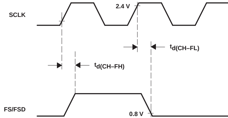
Figure 5-1. FS and FSD Timing
