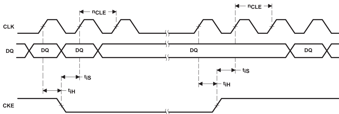
Figure 17. CLK-Suspend Operation
