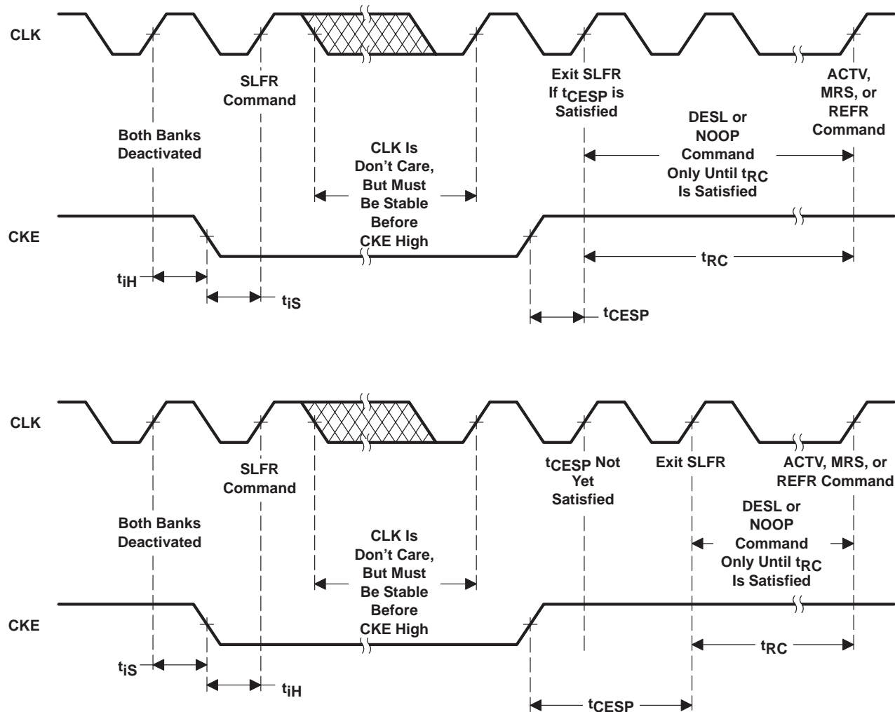
Figure 19. Self-Refresh Operation
