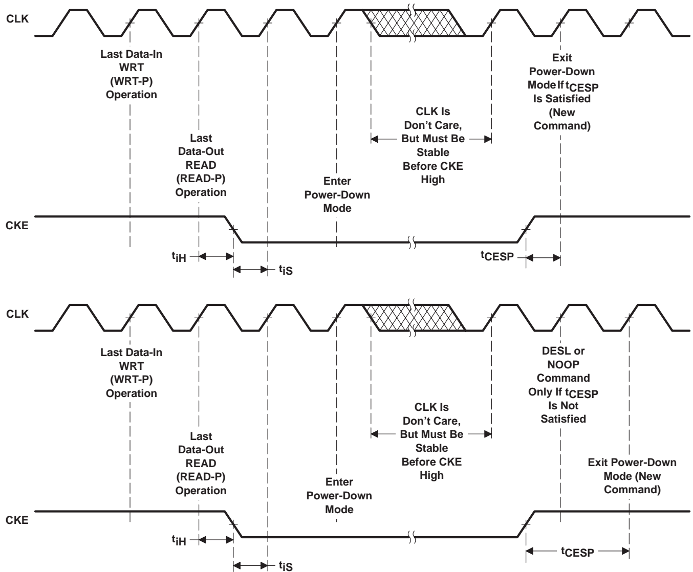
Figure 18. Power-Down Operation
