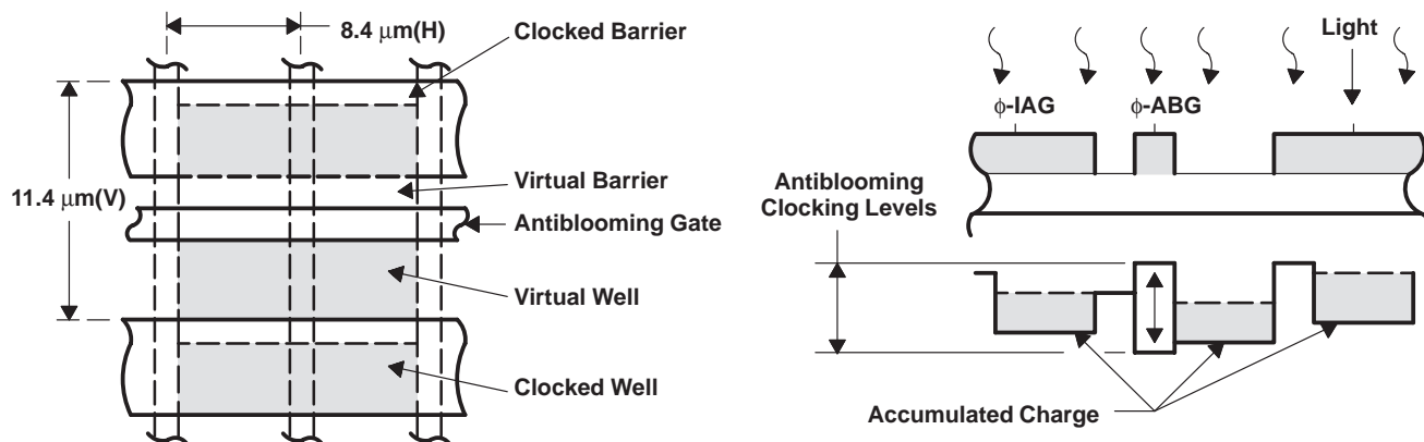
Figure 4. Charge-Accumulation Process
