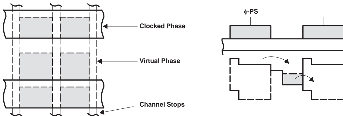
Figure 5. Charge-Transfer Process
