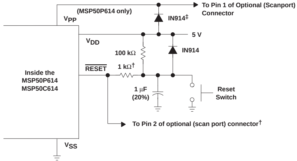
Figure 1–3. RESET Circuit
