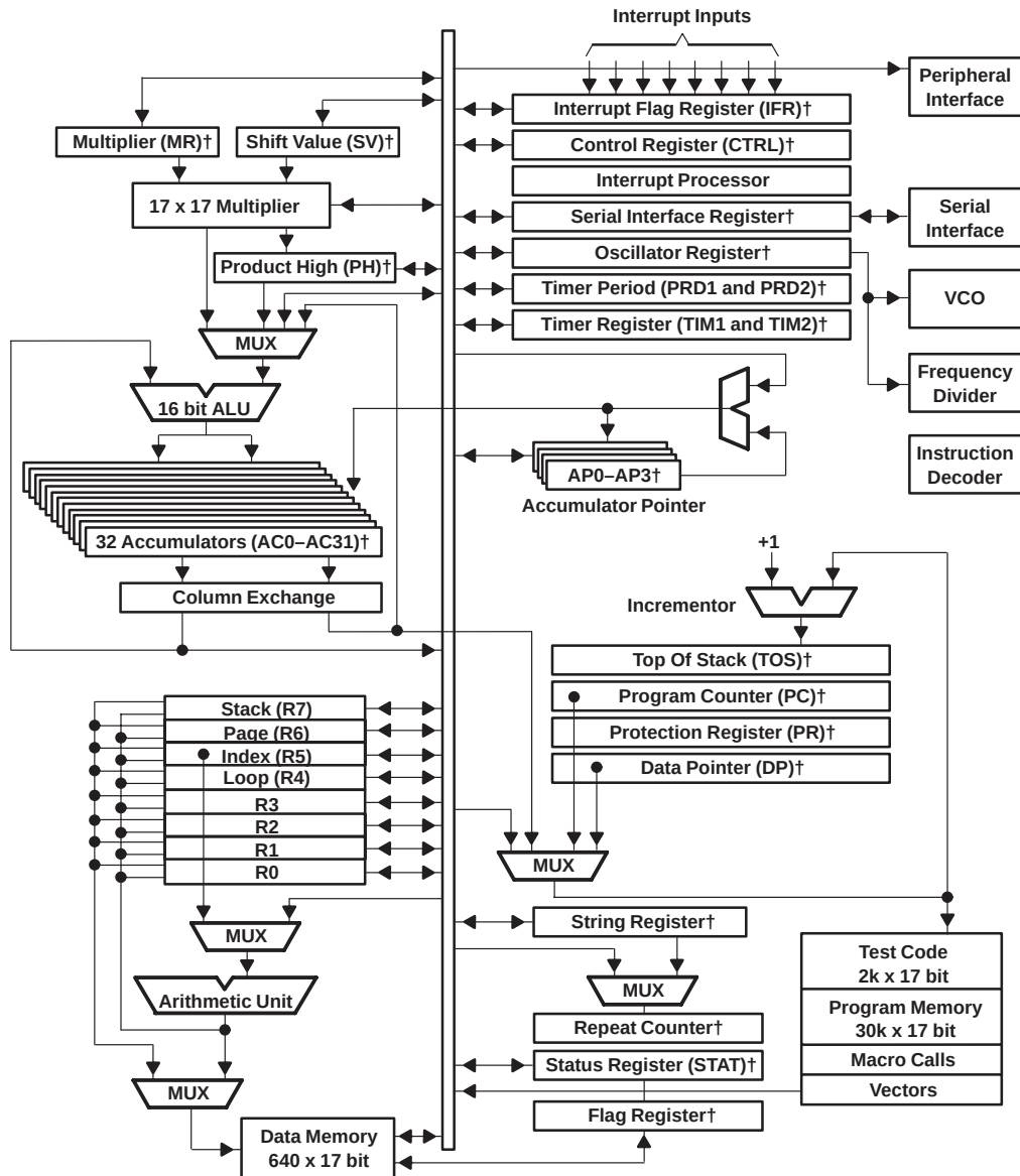
Figure 2–1. MSP50C614 Core Processor Block Diagram
