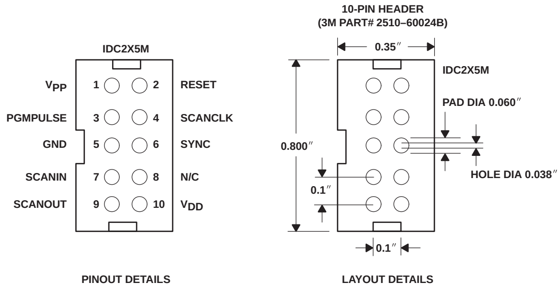
Figure 5–3. 10-Pin IDC Connector (top view looking at the board)
