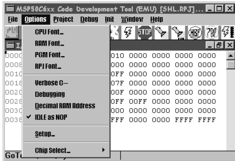
Figure 5–29. Miscellaneous Dialog
