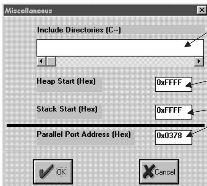
Figure 5–29. Miscellaneous Dialog
