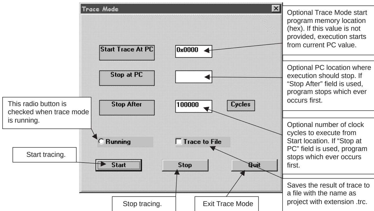
Figure 5–26. Trace Mode
