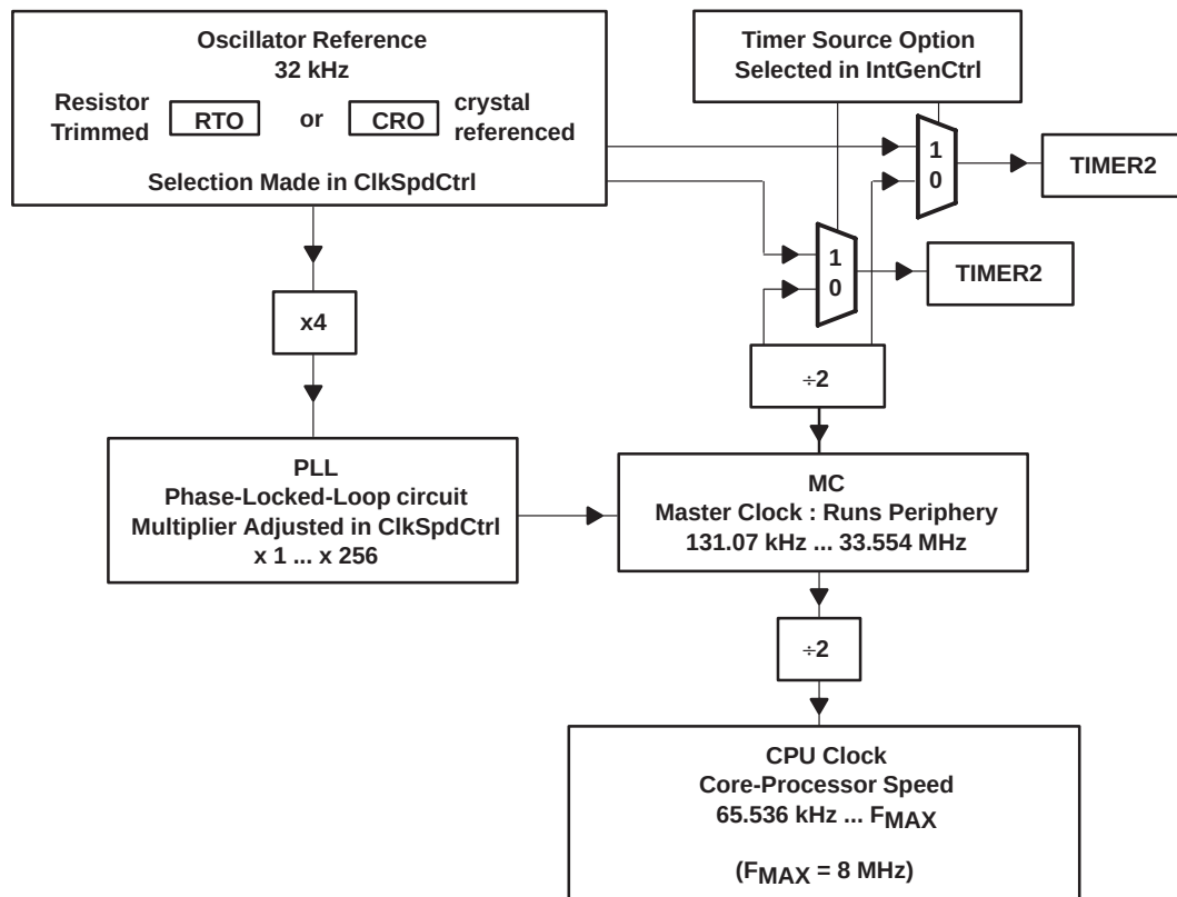
Figure 2–9. PLL Performance
