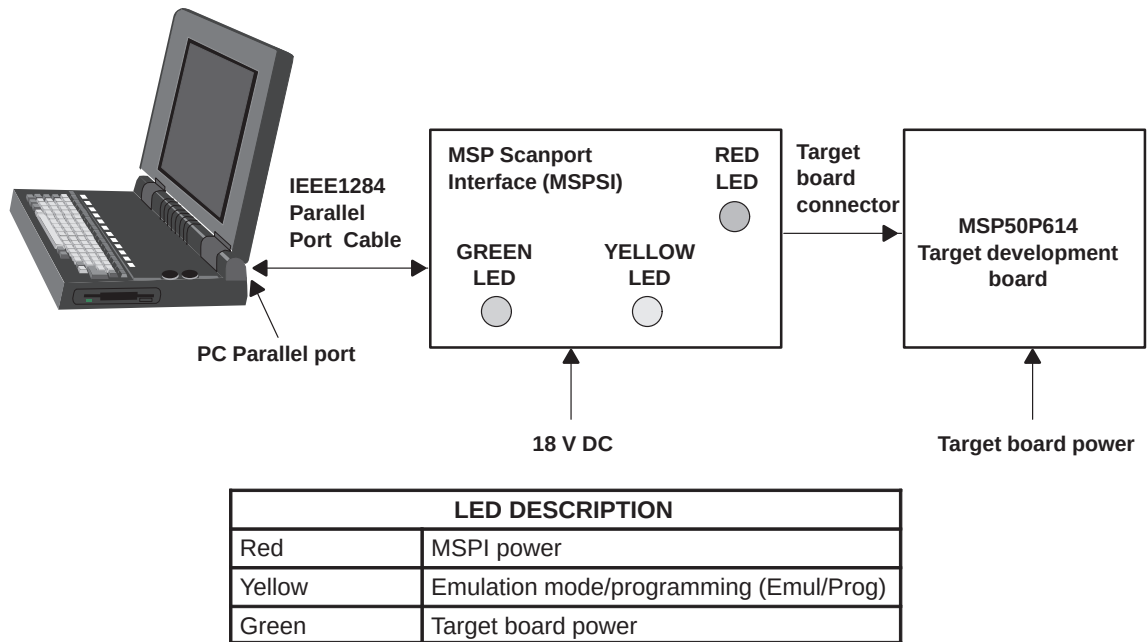
Figure 5–2. Hardware Installation
