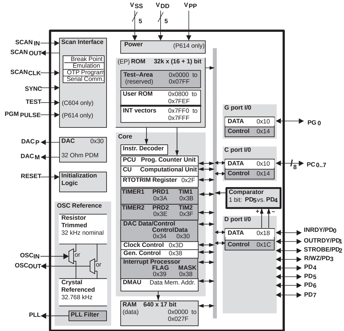
Figure B–1. MSP50C604 Block Diagram
