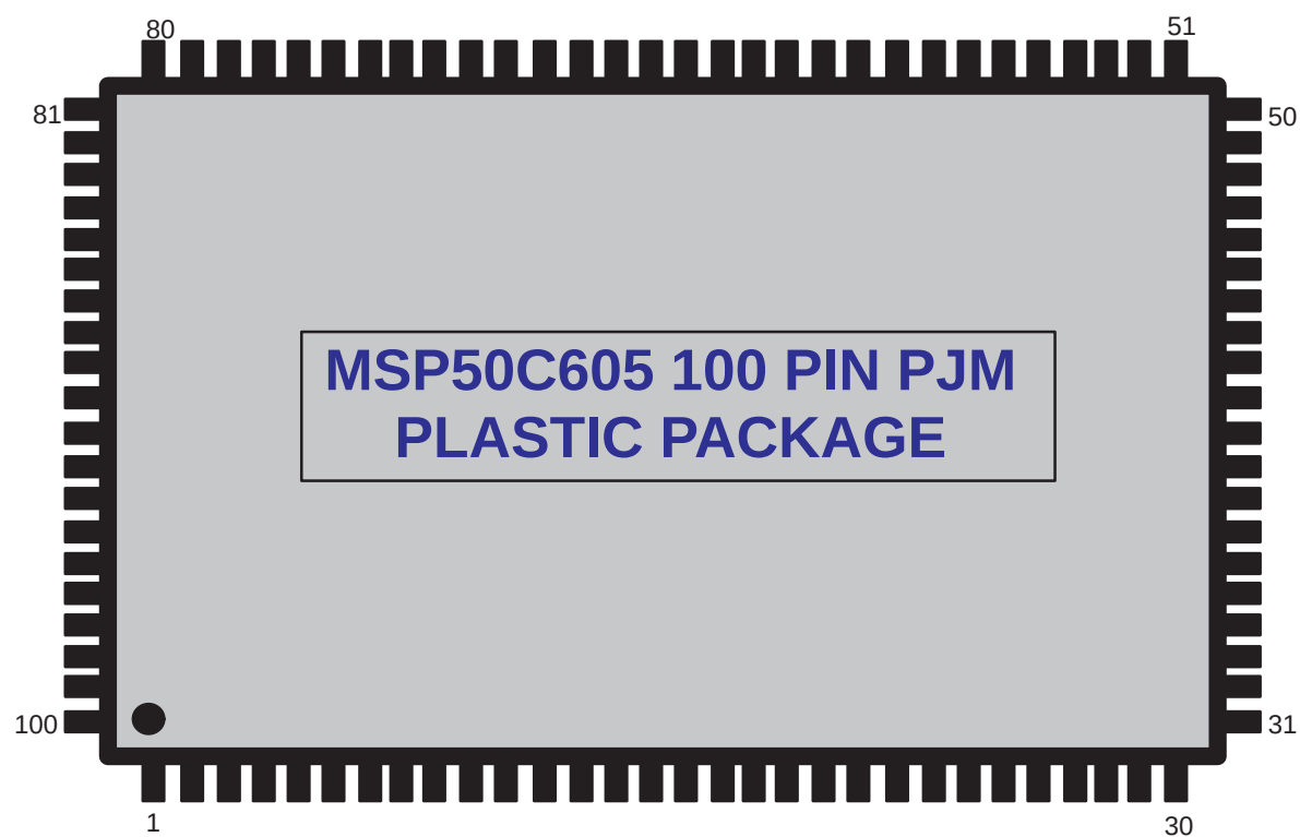
Figure A–3. MSP50C605 100-Pin PJM Package
