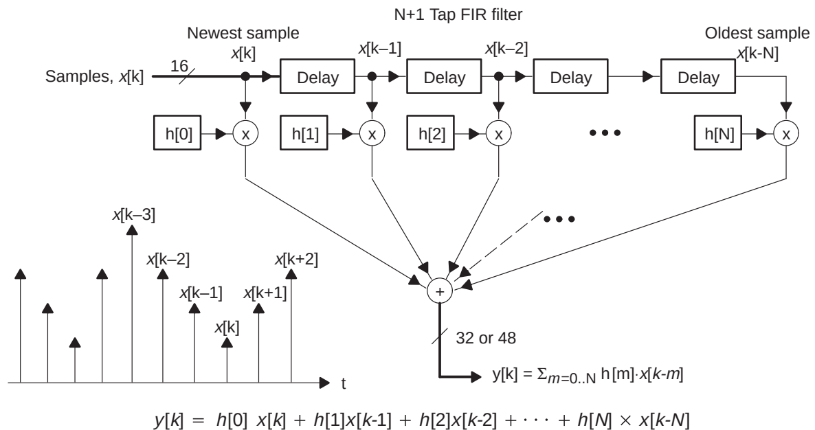
Figure 4–5. FIR Filter Structure
