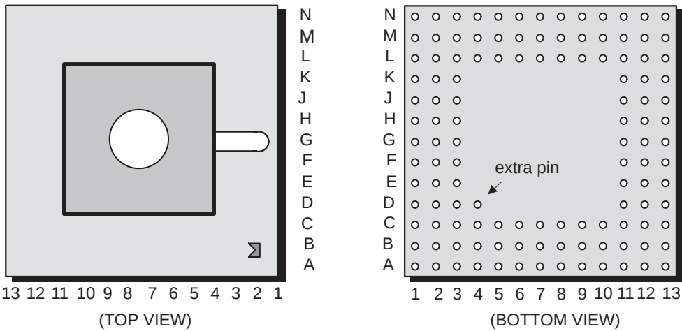
Figure 7–2. 120-Pin Grid Array Package for the Development Device, P614
