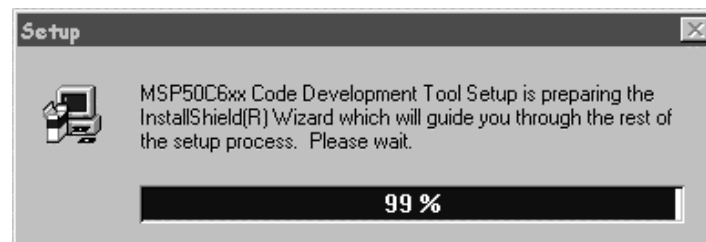
Figure 5–4. InstallShield Window
