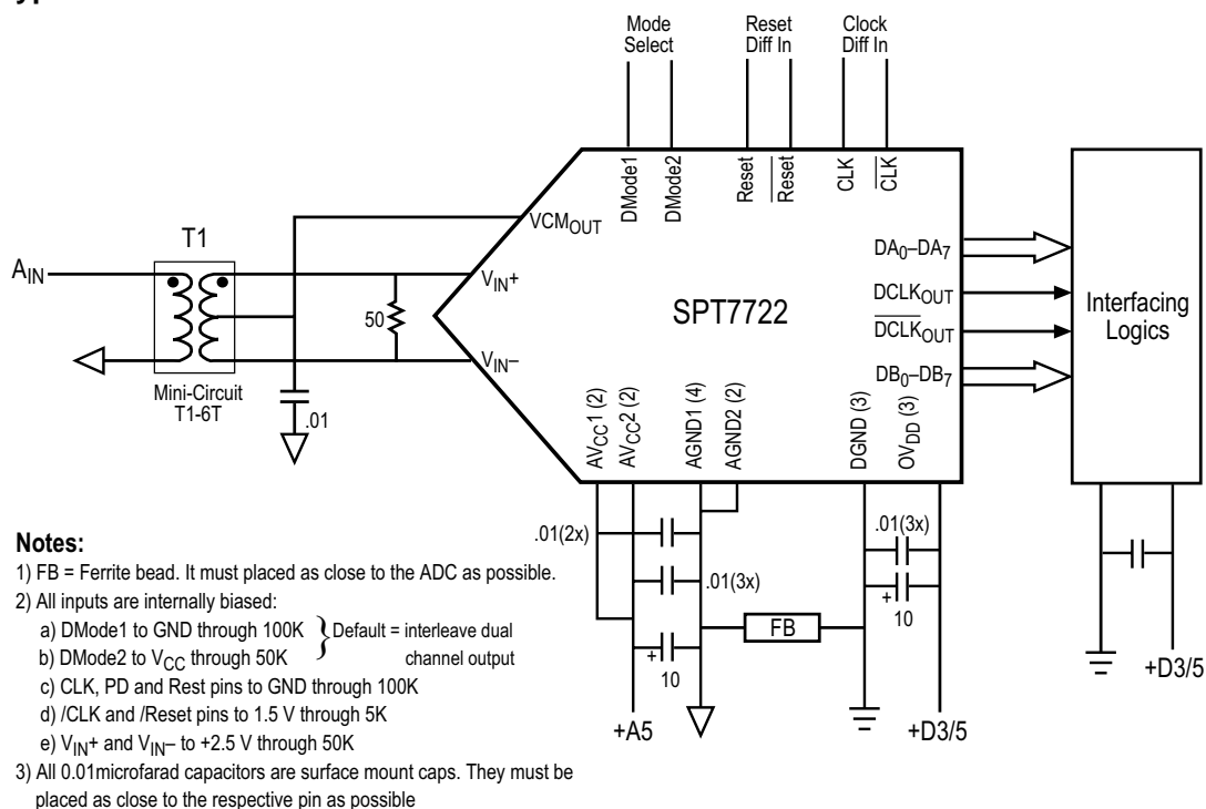
Figure 3 – Typical Interface Circuit
