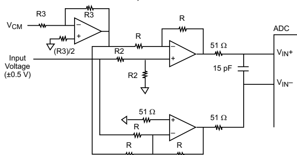
Figure 4 – DC-Coupled Single-Ended to Differential Conversion (power supplies and bypassing are not shown)
