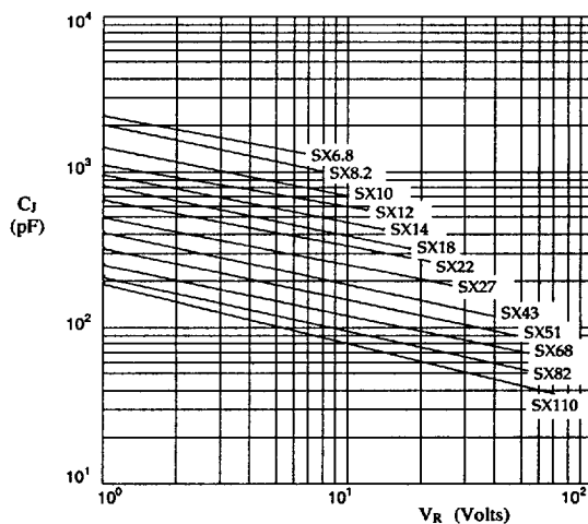
Fig 3. Typical junction capacitance versus reverse voltage.
