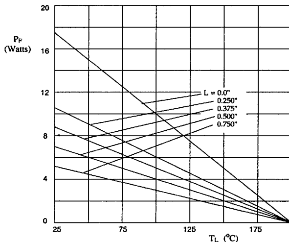
Figure 1. Maximum power versus lead temperature.
