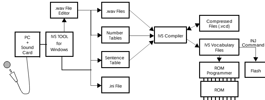
Figure 2-5: Creation of an IVS Vocabulary
