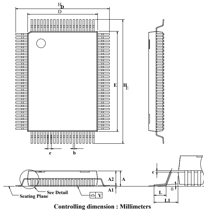
Figure 4-1: 100L PQFP (14x20x2.75mm footprint 3.2mm) IQC
