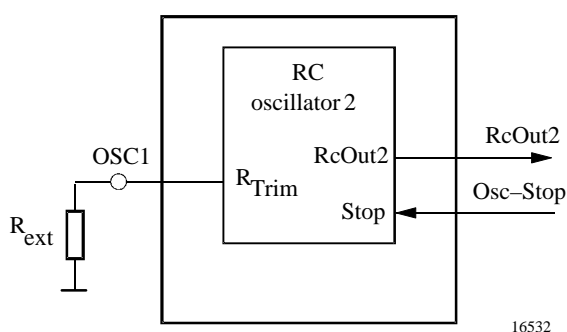
Figure 17. RC-oscillator 2
