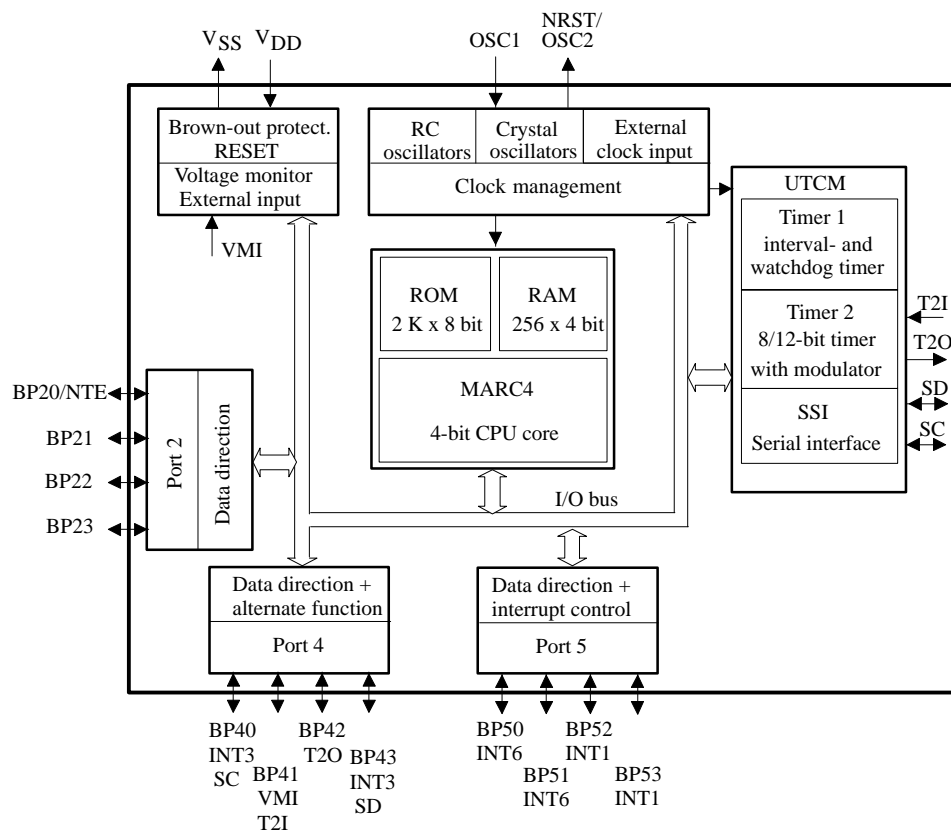
Figure 1. Block diagram of the T44C080-V
