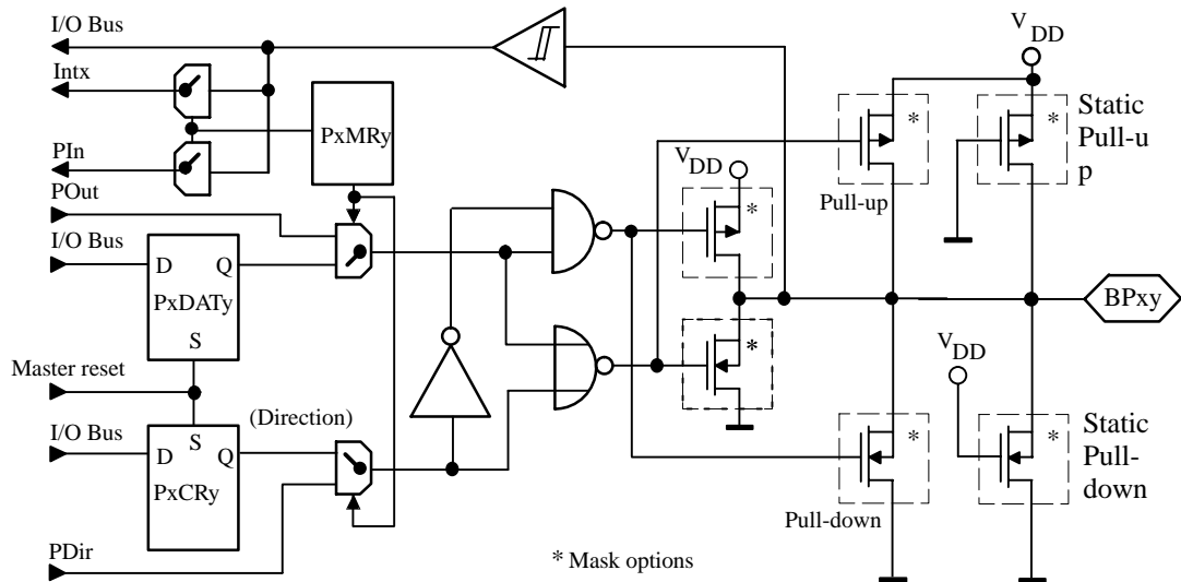
Figure 25. Bidirectional Port 4
