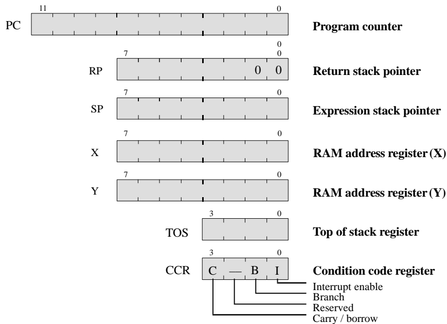
Figure 6. Programming model
