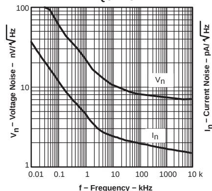
VOLTAGE AND CURRENT NOISE VS FREQUENCY
