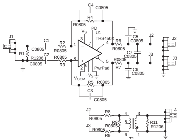
Simplified Schematic of the Evaluation Board. Power Supply Decoupling, V_{OCM} , and Power Down Circuitry Not Shown Figure 97
