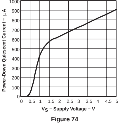
POWER-DOWN QUIESCENT CURRENT VS SUPPLY VOLTAGE
