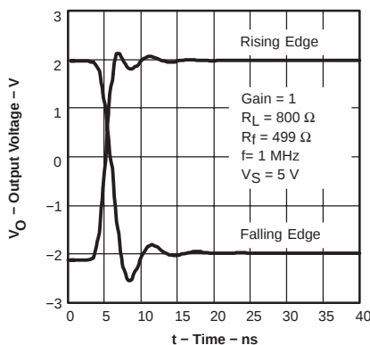
SETTLING TIME
