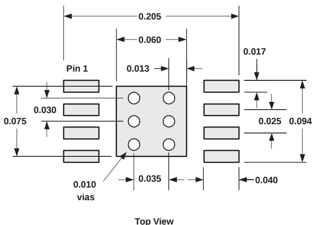
Figure 94. Views of Thermally Enhanced Package
