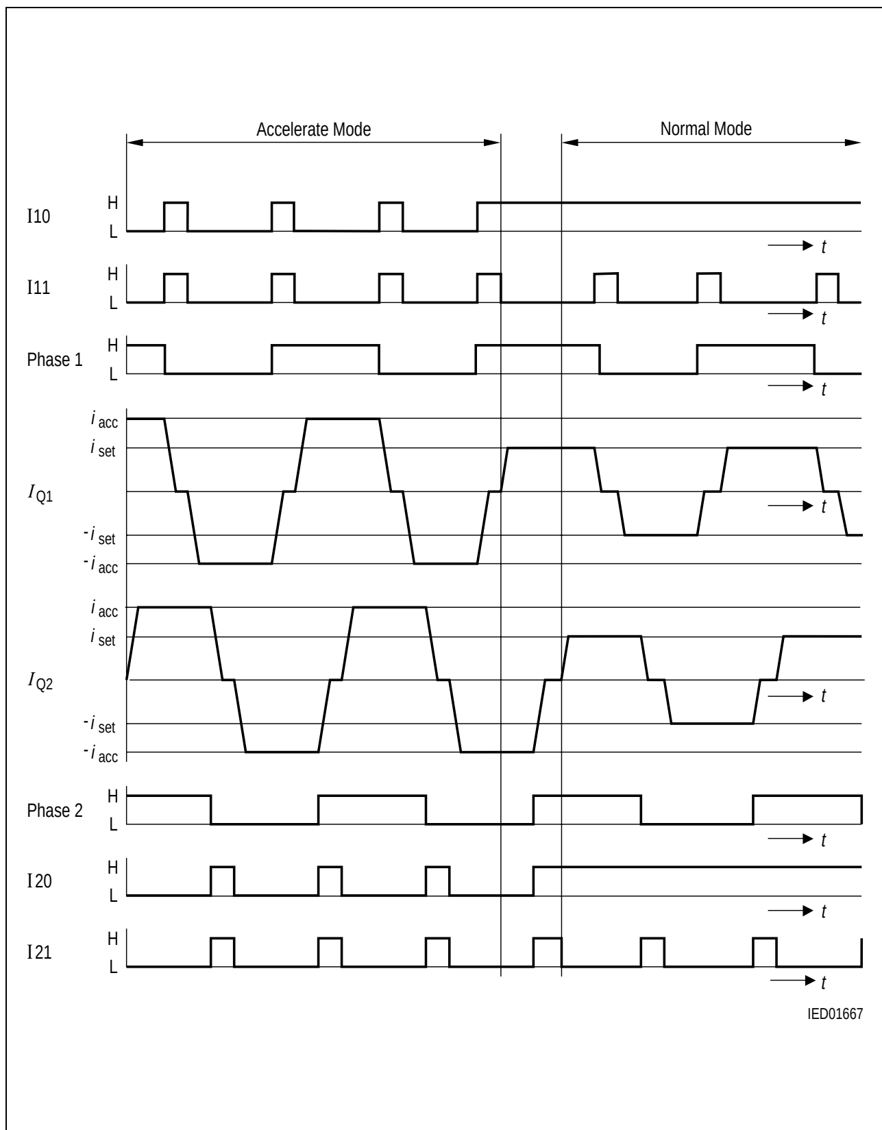
Figure 6 Half-Step Operation
