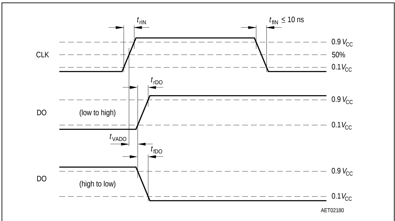
Figure 6 DO Valid Data Delay Time and Valid Time
