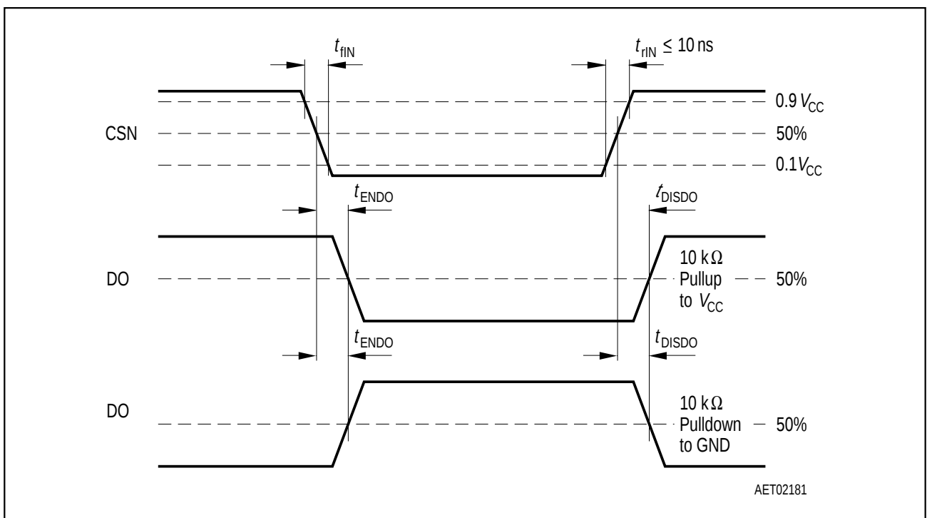
Figure 7 DO Enable and Disable Time
