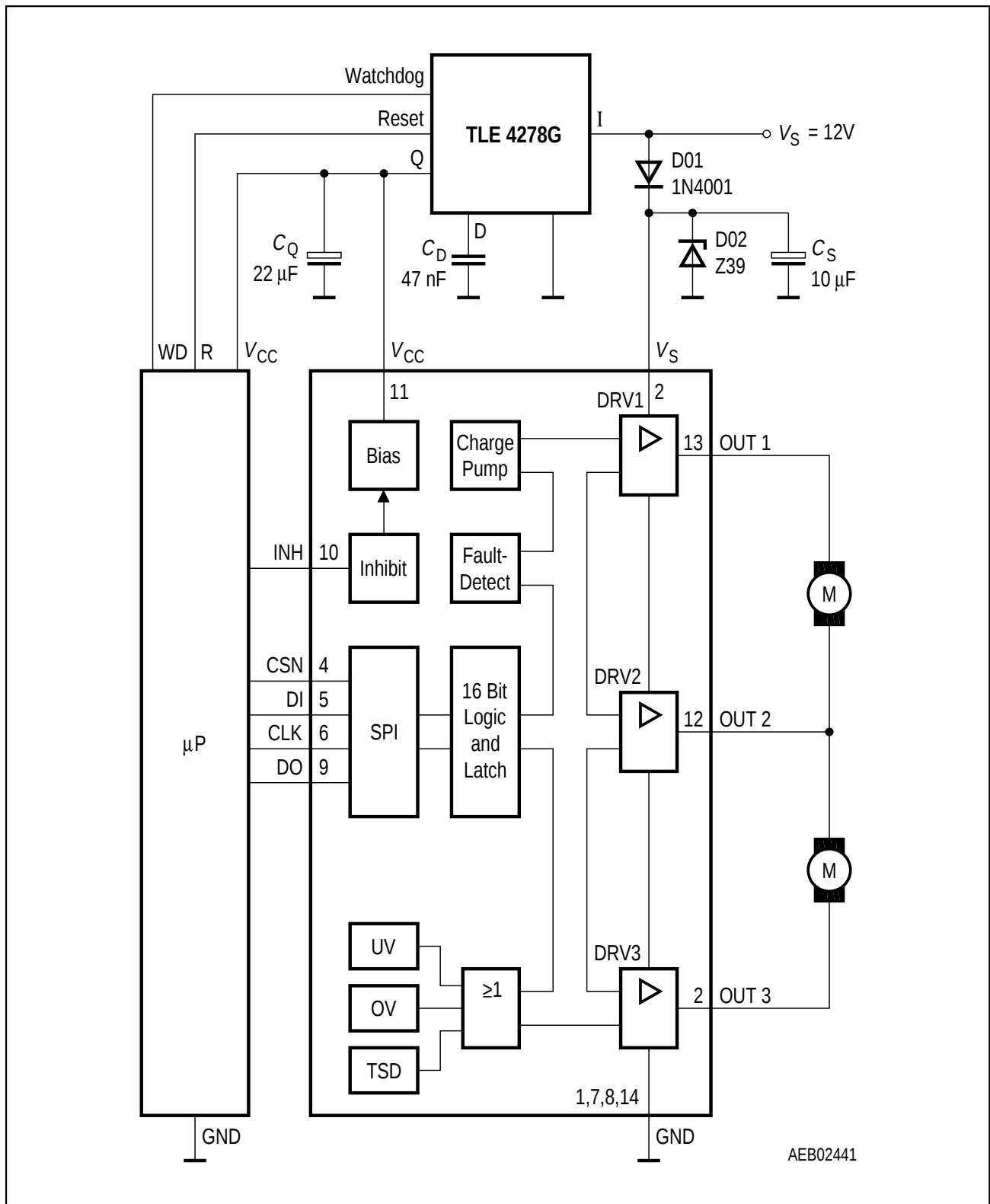
Figure 8 Application Circuit
