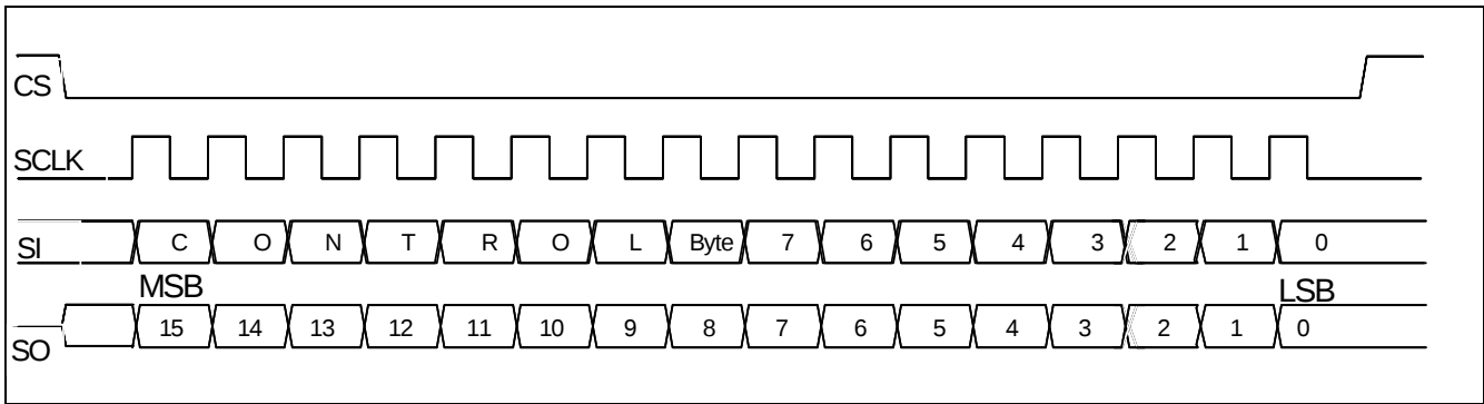
Figure 2: Serial Interface
