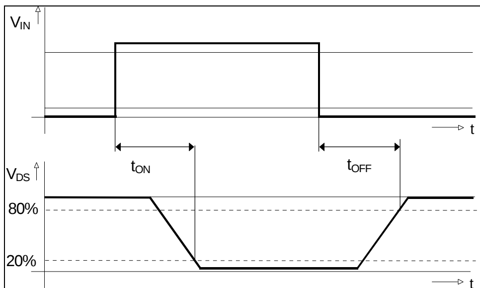
Figure 5: Power Outputs
