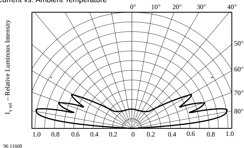
Figure 4 Rel. Luminous Intensity vs. Angular Displacement
