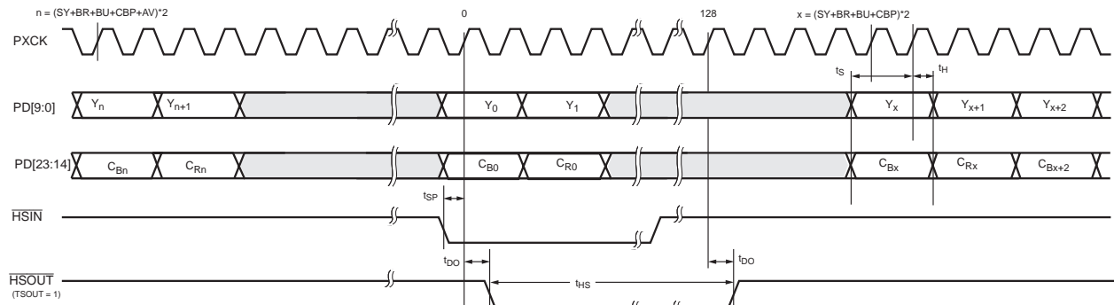
Figure 5. 20 bit 4:2:2 Input Format
