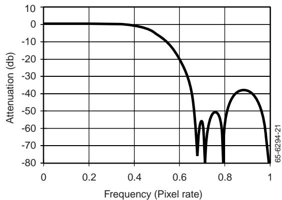
Figure 17. Interpolation Filter
