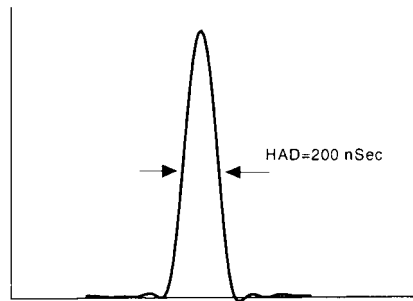
Figure 34. 2T Pulse
