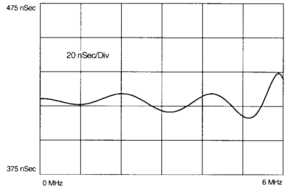
Figure 35. Group Delay
