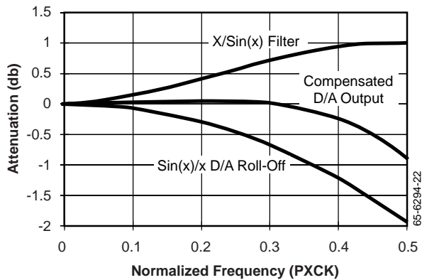
Figure 19. X/SIN(X) Filter
