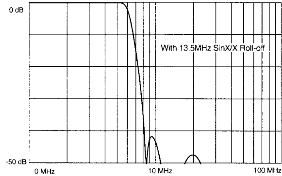
Figure 33. Stop Band
