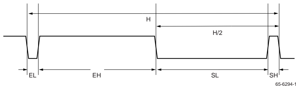
Figure 9. Horizontal Timing – Vertical Blanking
