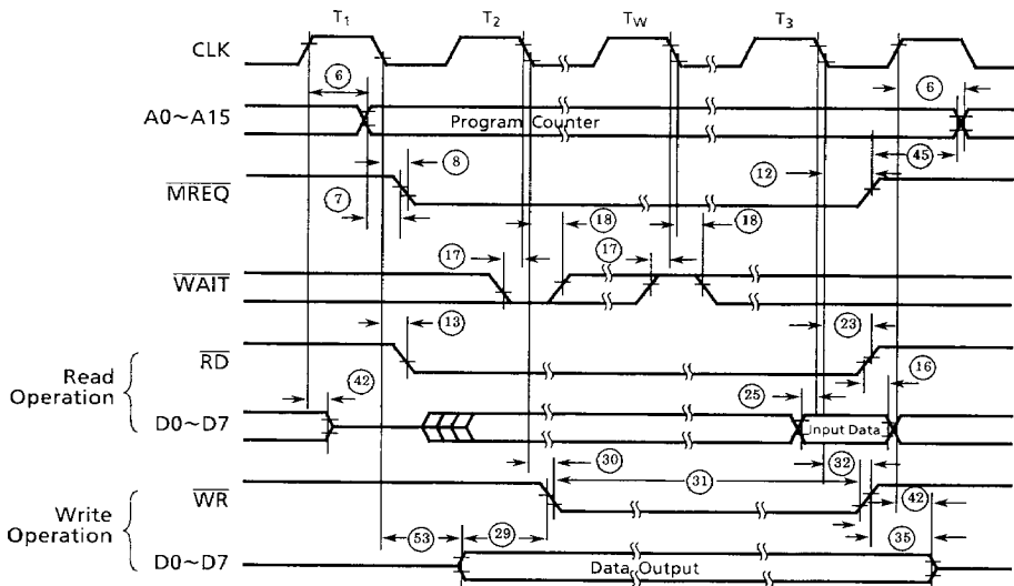
Figure 4.2 Memory Read/Write Cycle
