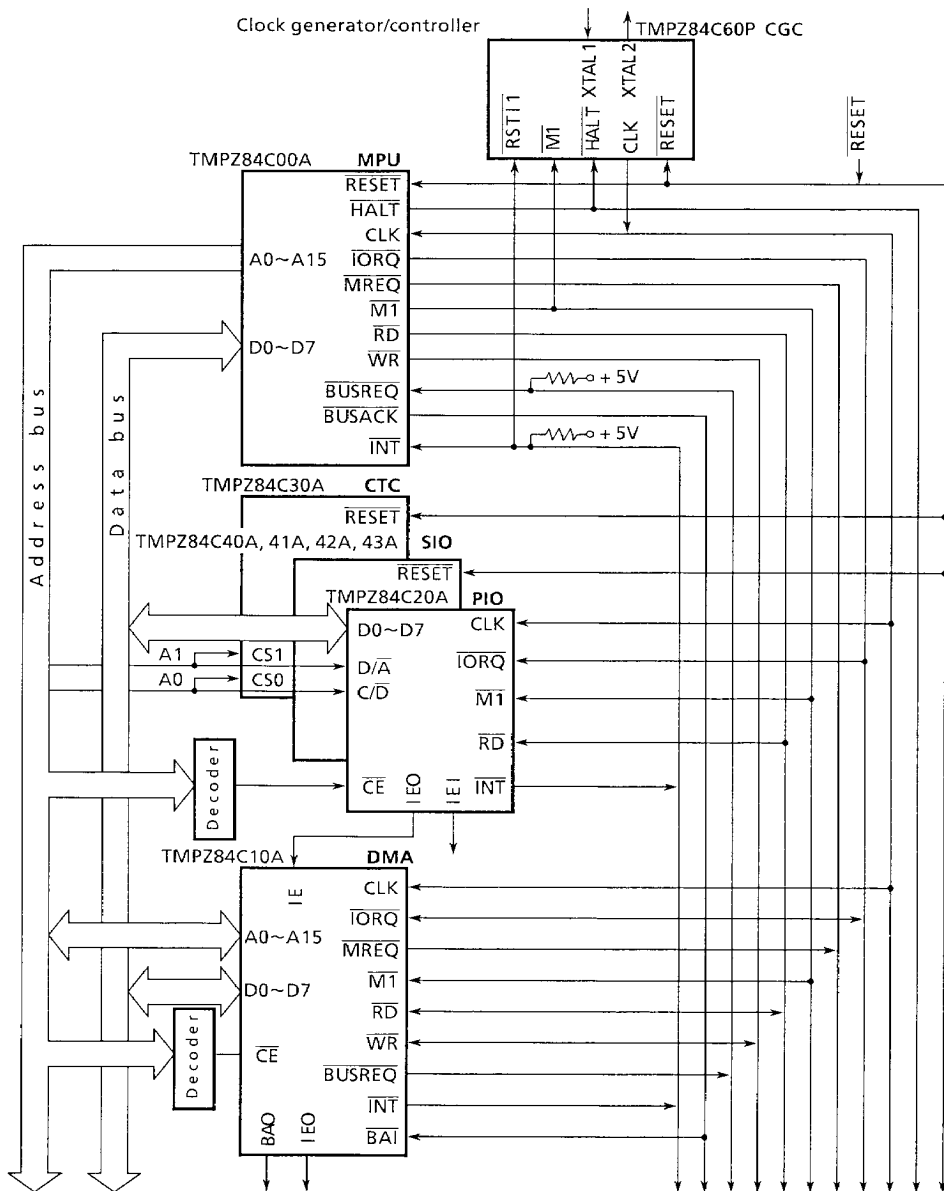
Figure 3.23 Example Connection with TLC5-Z80 family peripheral LSIs
