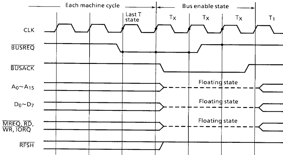
Figure 3.15 Bus Request and Bus Acknowledge Timing
