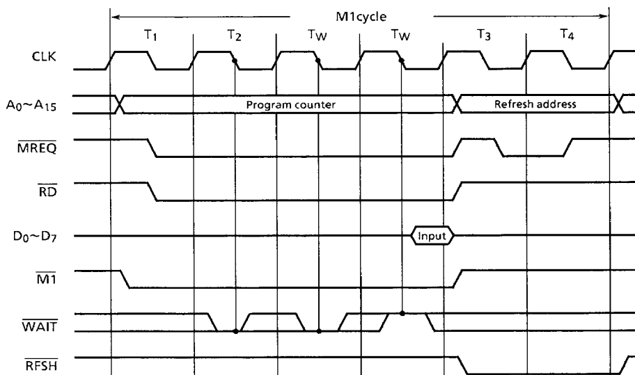
Figure 3.12 Opcode Fetch Timing Including Wait State
