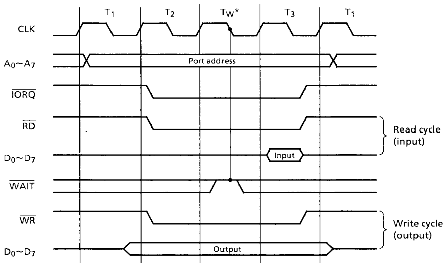
Figure 3.14 I/O Operating Timing
