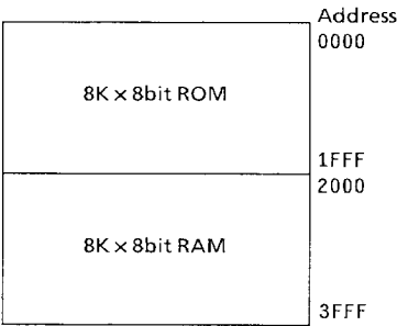
Figure 3.21 Address Assignment
