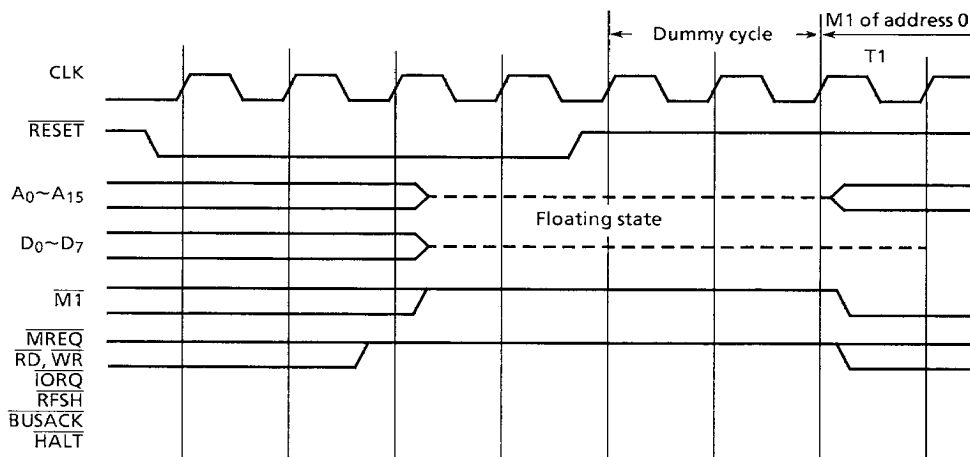
Figure 3.20 Reset Timing
