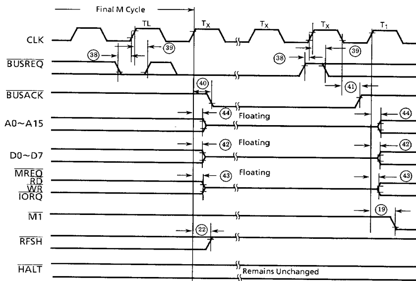
Figure 4.5 Non-maskable Interrupt Request Cycle
