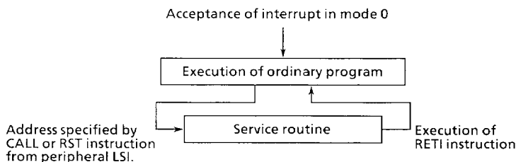
Figure 3.6 Interrupt Processing in Mode 0
