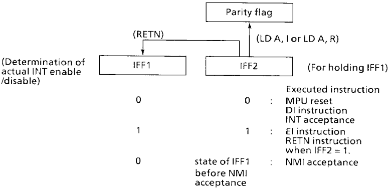
Figure 3.4 Interrupt Enable Flip-Flop (IFF)
