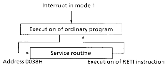
Figure 3.7 Interrupt Processing in Mode 1
