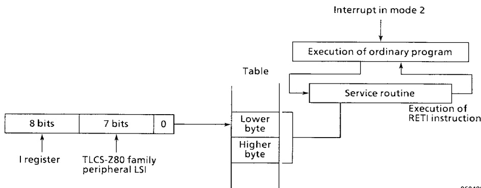
Figure 3.8 Interrupt Processing in Mode 2
