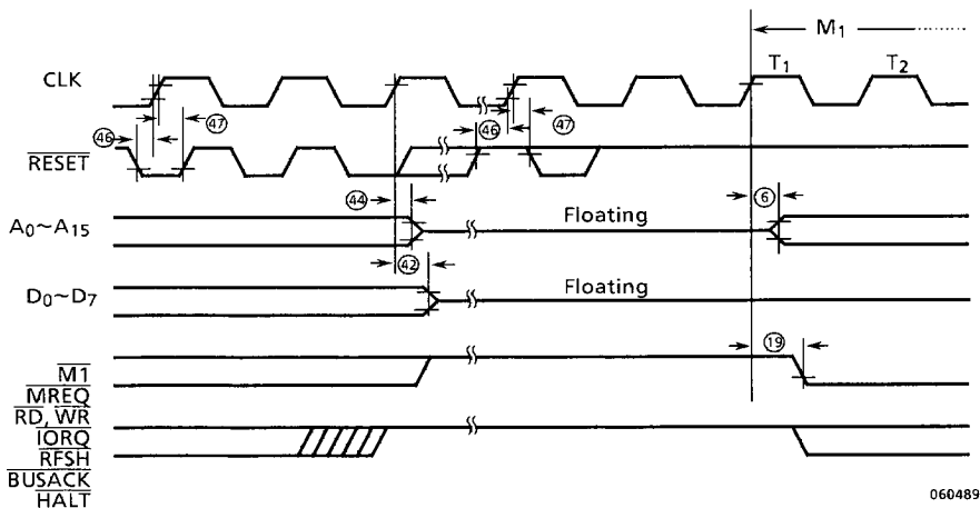
Figure 4.8 Reset Cycle
