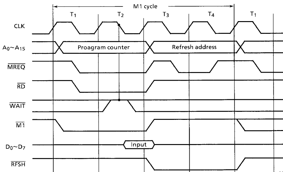
Figure 3.11 Opcode Fetch Timing
