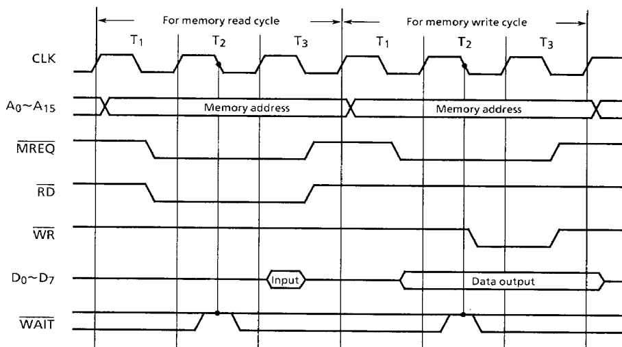
Figure 3.13 Memory Read/Write Cycle Timing
