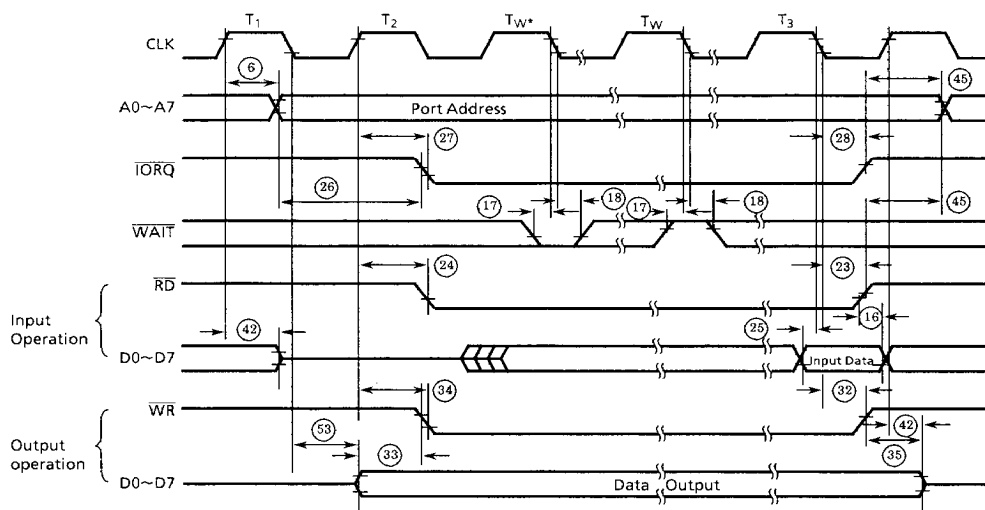
Figure 4.3 Input/Output Cycle
