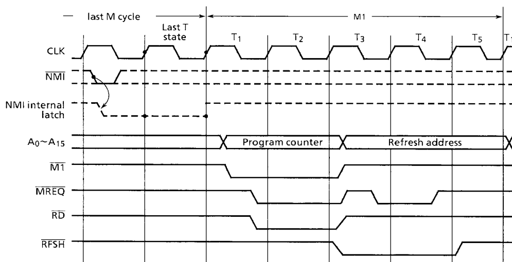
Figure 3.17 Non-Maskable Interrupt Acknowledge Timing
