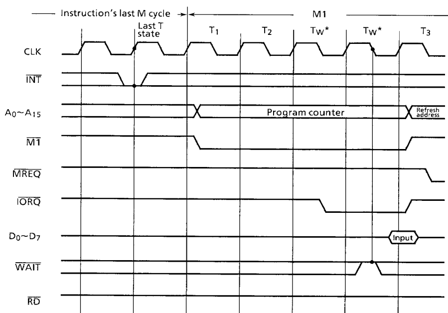
Figure 3.16 Maskable Interrupt Acknowledge Timing
