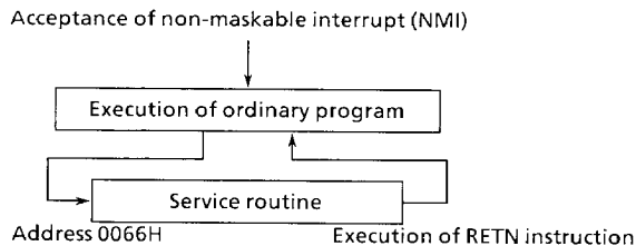
Figure 3.5 Non-Maskable Interrupt Processing
