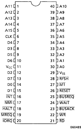
Figure 2.1 DIP, SOP Pin Assignment
