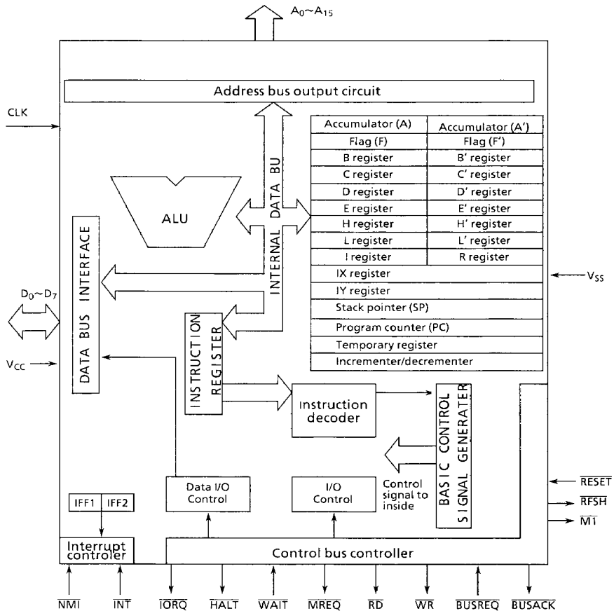
Figure 3.1 Block Diagram
