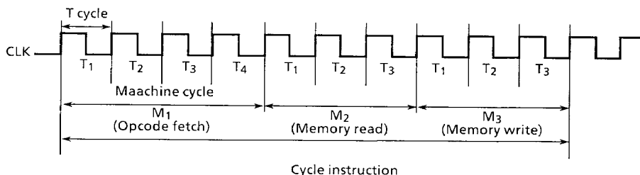
Figure 3.9 Example of MPU Basic Timing (3-Machine-Cycle Instruction)
