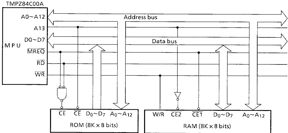
Figure 3.22 Example Connection with Memories
