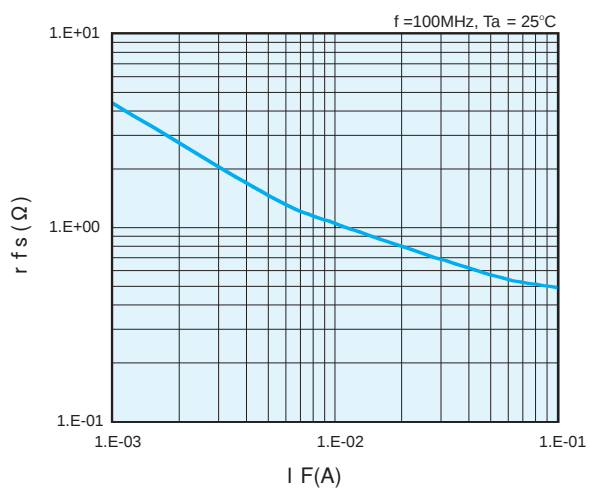
Forward Series Resistance vs. Forward Current
