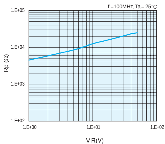
Parallel Resistance vs. Reverse Voltage
