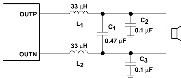
Figure 33. Typical LC Output Filter, Cutoff Frequency of 41 kHz, Speaker Impedance = 8 Ω
