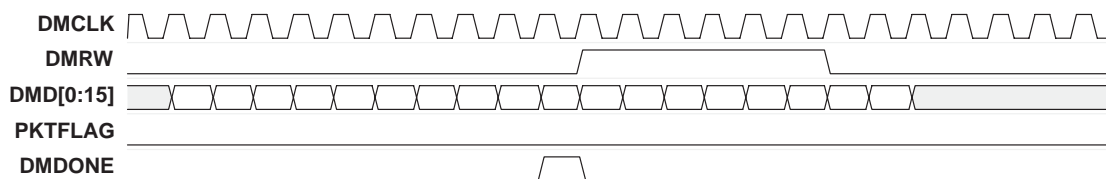
Figure 5–28. Asynchronous Block Receive With Automatic Header and Trailer Removal at 400 Mbps
