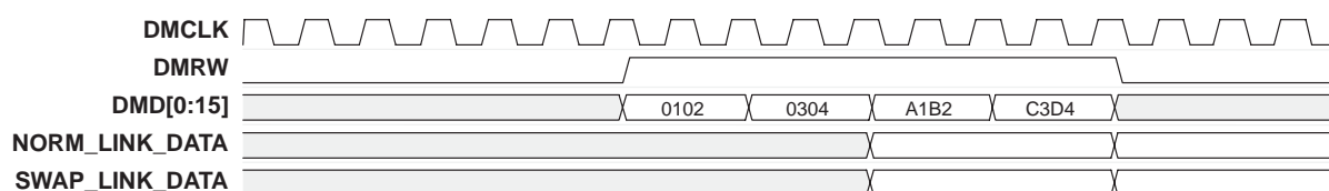
Figure 5–30. Endian Swapping in Word Mode
