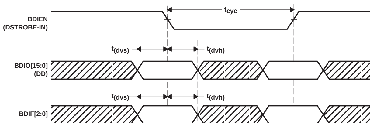
Figure 9–10. ATAPI Read
