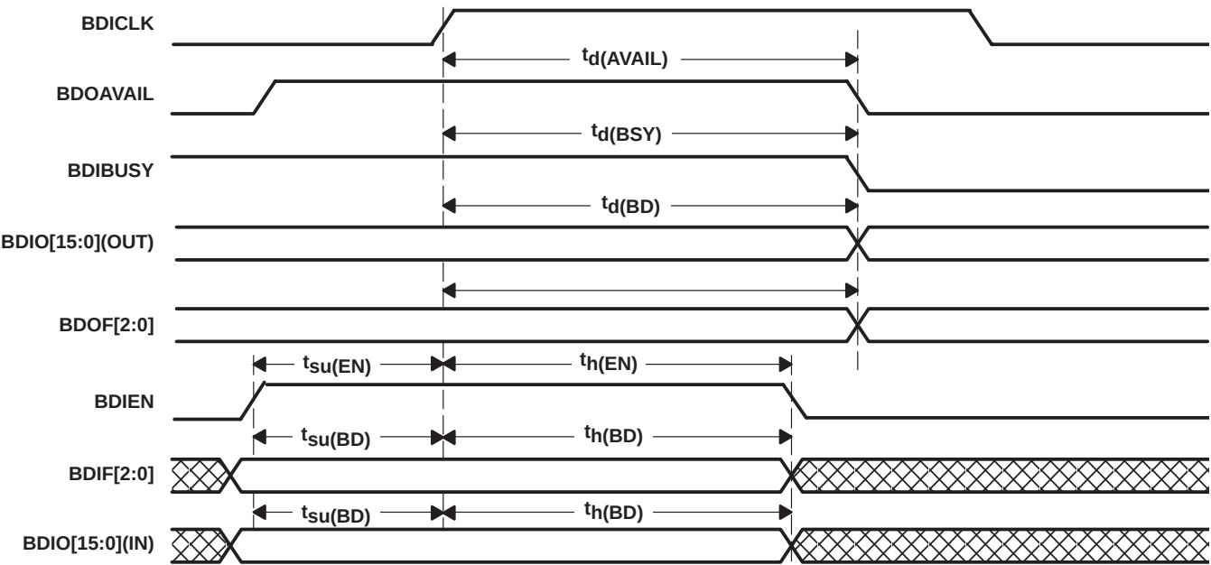
Figure 9–1. Synchronous Mode
