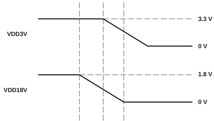
Figure 12–8. Power-Down Sequence
