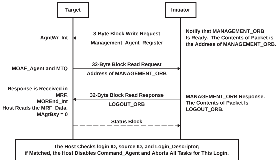
Figure 7–4. Logout Process
