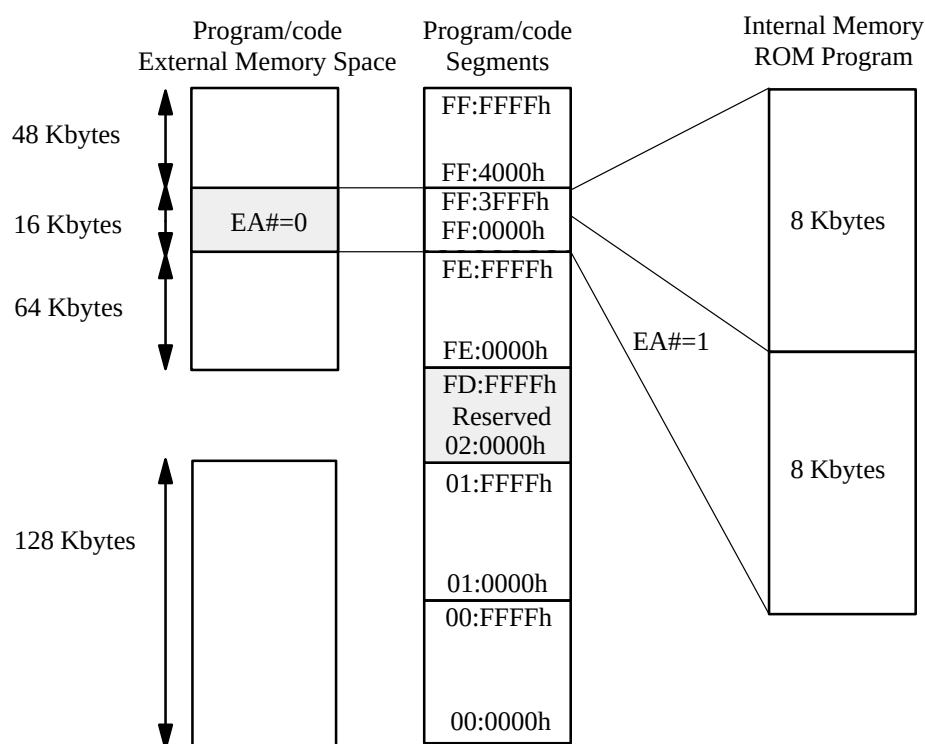
Figure 1.9. Programmable Memory Mapping
