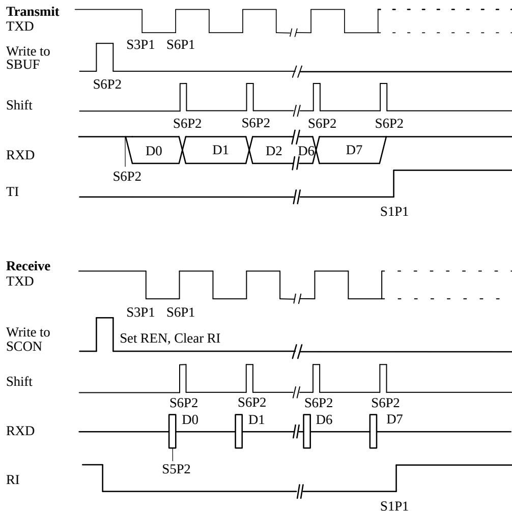
Figure 4.2. Mode 0 Timings
