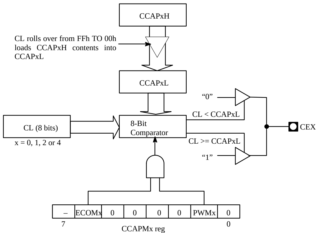
Figure 5.5. PWM Mode
